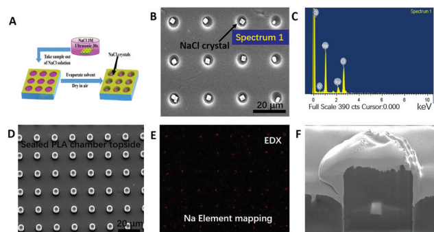
Fig. 3 Encapsulation of small hydrophilic molecules within air bubbles in PLA thin films and proof of successful encapsulation. (A) Scheme of NaCl crystal encapsulation within hydrophobic PLA microchambers. (B) SEM image of PLA@NaCl crystals in microchambers before sealing (PLA m\% = 2%), the size of NaCl crystals is 1 \pm 0.2 \mu\text{m} . (C) EDX analysis of NaCl crystals loaded into PLA chambers. (D) SEM image of the sealed PLA@NaCl microchambers (PLA m\% = 1%). (E) EDX mapping analysis of PLA@NaCl microchambers, proving that NaCl is within the chambers of (D). (F) Focused ion beam (FIB) image of a half-cut and sealed PLA@NaCl microchamber (PLA m\% = 2%), uneven wall thickness from PLA melting upon FIB cutting.
