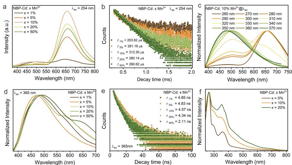
Fig. 5 (a) Prompt emission spectra and (b) corresponding decay curves for the red emissions at 660 nm in NBP-Cd:xMn 2+ under excitation at 254 nm. (c) Excitation-dependent emission spectra of the NBP-Cd:10%Mn 2+ sample. (d) Prompt emission spectra and (e) corresponding decay curves for high-energy yellow-green emissions in NBP-Cd:xMn 2+ under excitation at 365 nm. (f) UV-vis absorption spectra of NBP-Cd:xMn 2+ ( x = 0, 10%, and 20%).
