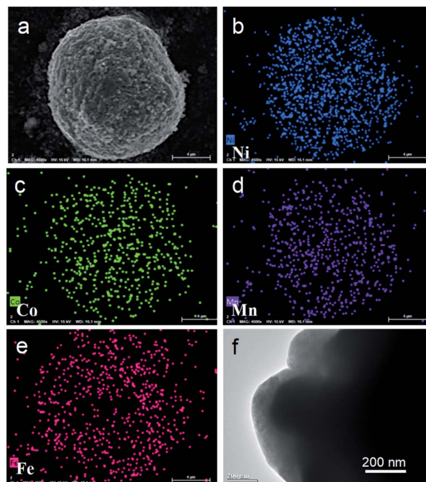
Fig. 3 (a–e) EDS elemental mapping of NCM@LFP 100, and (f) TEM image of NCM@LFP 100.
