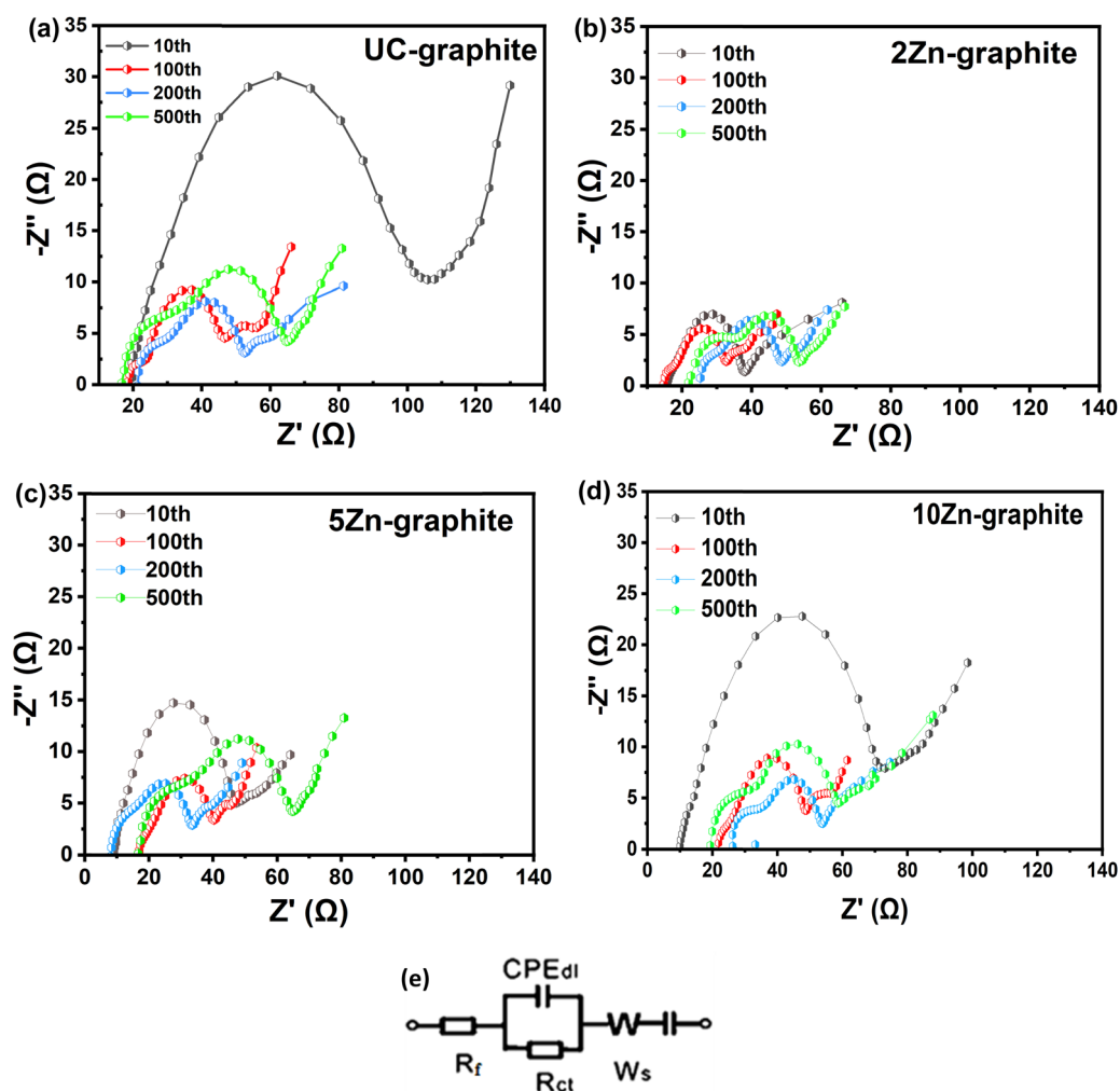
Fig. 4 Nyquist plots of anode samples tested at a 1C rate with a potential range of 0.1–3.0 V at the 10th, 100th, 200th, and 500th charge/discharge cycles for (a) UC-graphite, (b) 2Zn-graphite, (c) 5Zn-graphite, and (d) 10Zn-graphite, and (e) the electrical equivalent circuit model.
