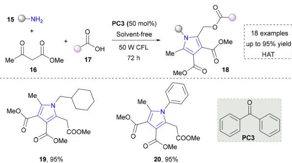
Scheme 3 Three-component reaction for complex pyrrole synthesis.
