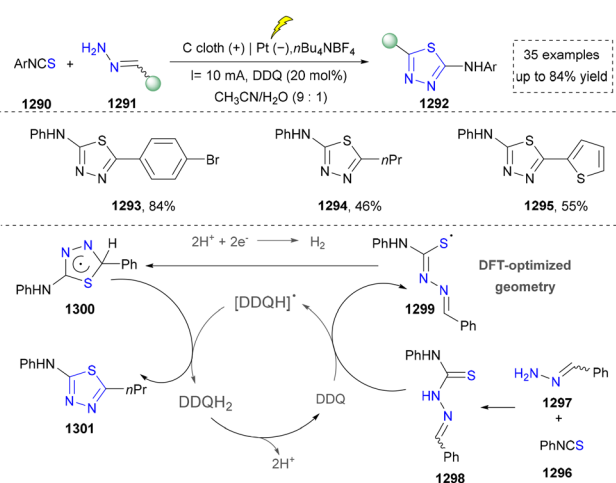
Scheme 135 Electrochemical oxidative synthesis of 1,3,4-thiadiazoles.
