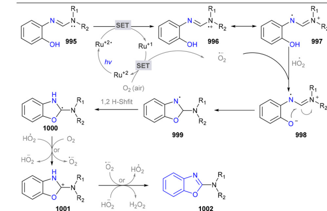
Scheme 105 Visible-light-triggered oxidation for the synthesis of 2-aminobenzoxazoles.
