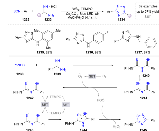
Scheme 130 Semi-heterogeneous photosynthesis of 5-amino-1,2,4-thiadiazoles.
