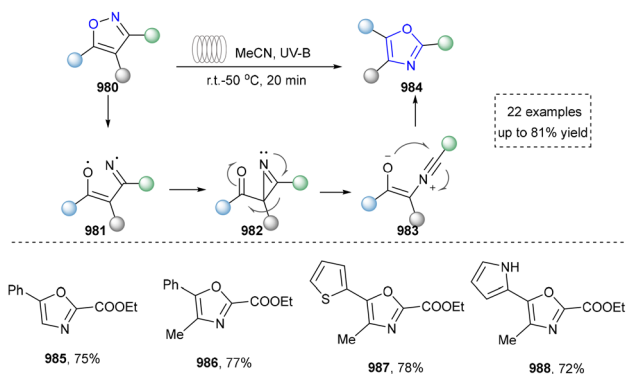
Scheme 104 Access to diverse oxazoles from isoxazoles enabled by continuous-flow photoisomerization.
