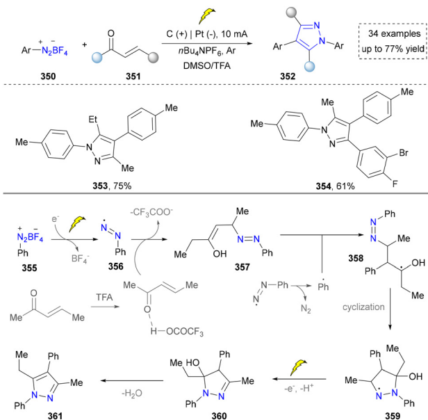
Scheme 40 Electrochemical synthesis of pyrazoles via a radical cyclization cascade.
