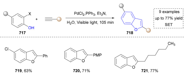
Scheme 77 The formation of benzofurans by the cyclisation of ortho -halophenols and terminal alkynes.
