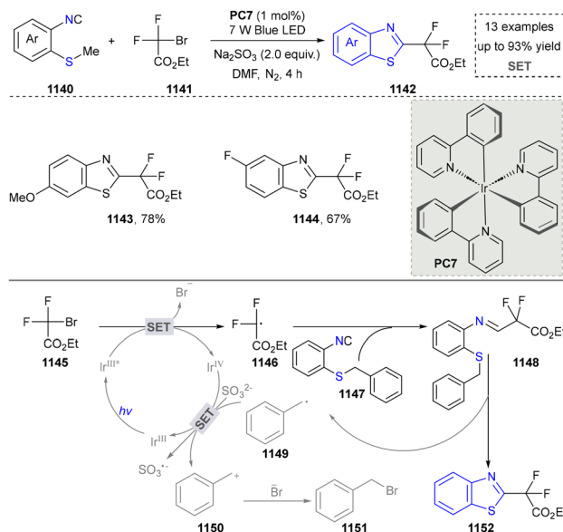
Scheme 121 Photocatalytic cyclization for the synthesis of 2-CF 2 /CF 3 -containing benzothiazoles.
