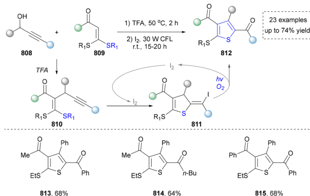
Scheme 86 Synthesis of 2,4-diacyl thiophenes from \alpha -oxo-ketene dithioacetals and propargylic alcohols.
