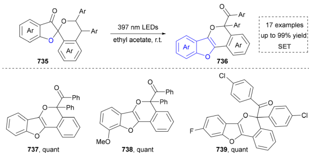
Scheme 79 Electrocyclic reactions of 1,8-dioxatetraene.
