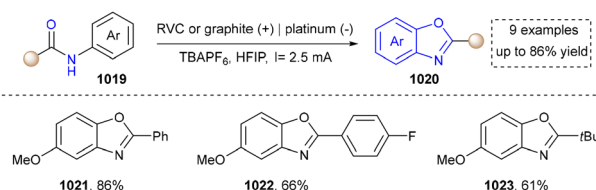
Scheme 108 Electrochemical synthesis of benzoxazoles from anilides.
