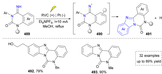
Scheme 52 Synthesis of benzimidazoles through the anodic N–H bond cleavage.
