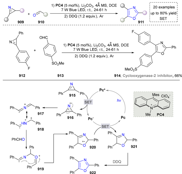
Scheme 96 [3+2] cycloaddition/oxidative aromatization sequence to afford oxazoles.
