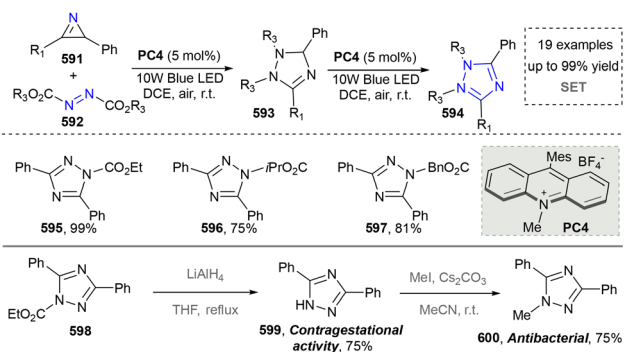
Scheme 64 Visible-light-induced cyclization reactions for the synthesis of 1,2,4-triazoles.
