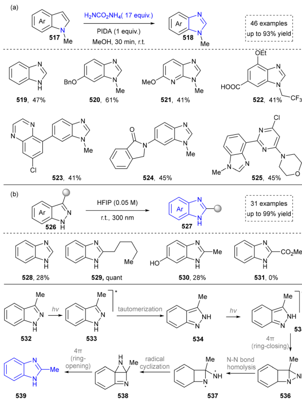
Scheme 55 (a) Access to benzimidazole derivatives from indoles via carbon-nitrogen atom exchange. (b) Photochemical conversion of indazoles into benzimidazoles.
