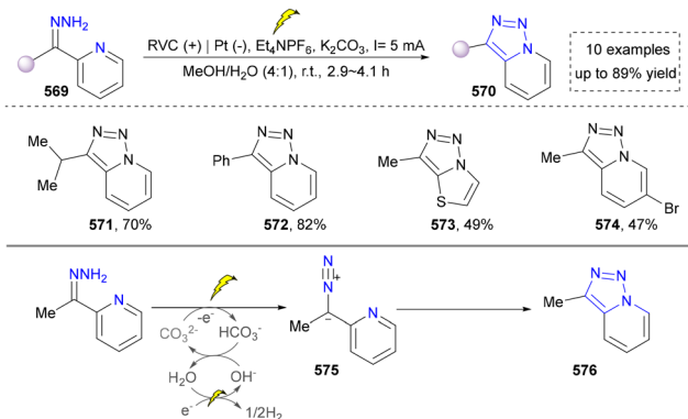
Scheme 60 Electrochemical synthesis of 1,2,3-triazoles through dehydrogenative cyclization.
