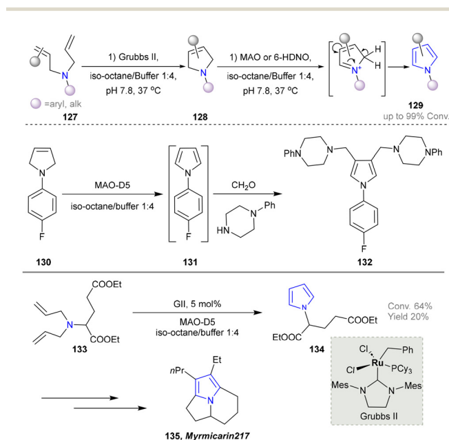
Scheme 12 Chemoenzymatic cascade process for the synthesis of pyrroles using MAO-N.
