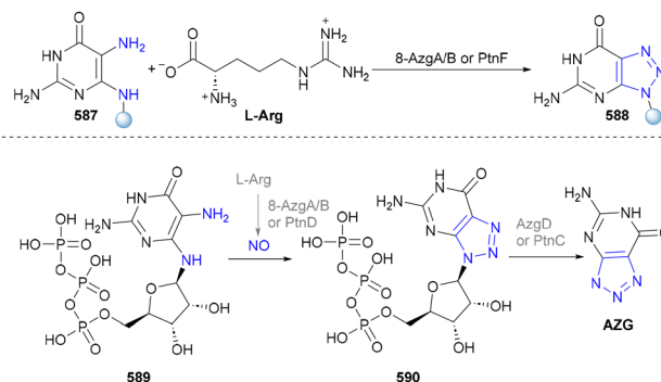
Scheme 63 Enzymatic synthesis of the triazolopyrimidine scaffold.
