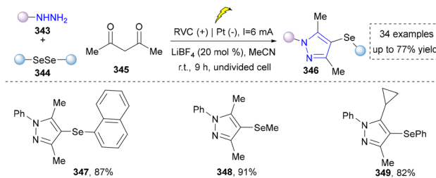
Scheme 39 Electrochemical synthesis of 4-selanylpyrazoles.
