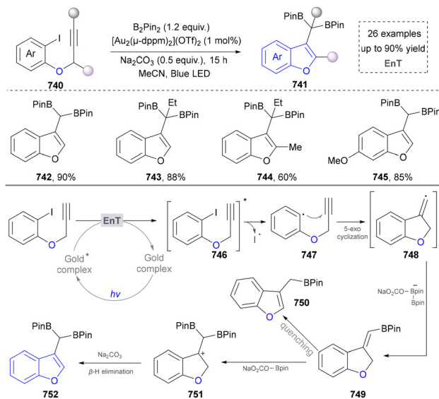
Scheme 80 Visible-light-induced gem -diborylation for the synthesis of benzofurans.
