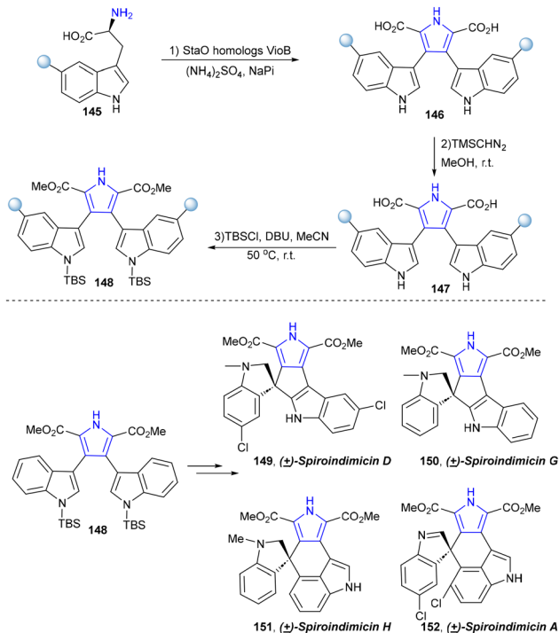
Scheme 14 Biomimetic total synthesis of the spiroindimicin family.
