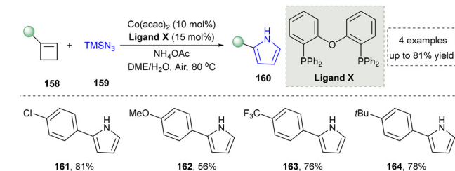
Scheme 16 Cobalt-catalyzed nitrogen-atom insertion for the pyrrole formation.
