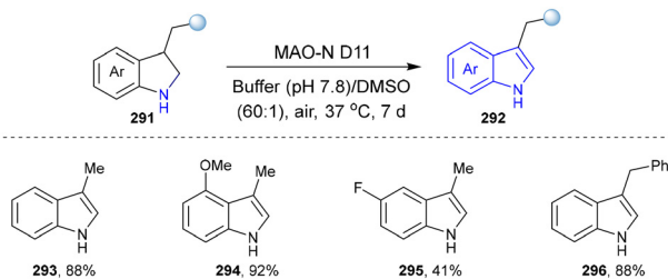
Scheme 31 Enzymatic synthesis of the indole derivatives catalysed by MAO.
