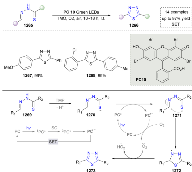
Scheme 133 Visible-light-promoted synthesis of 1,3,4-thiadiazoles.
