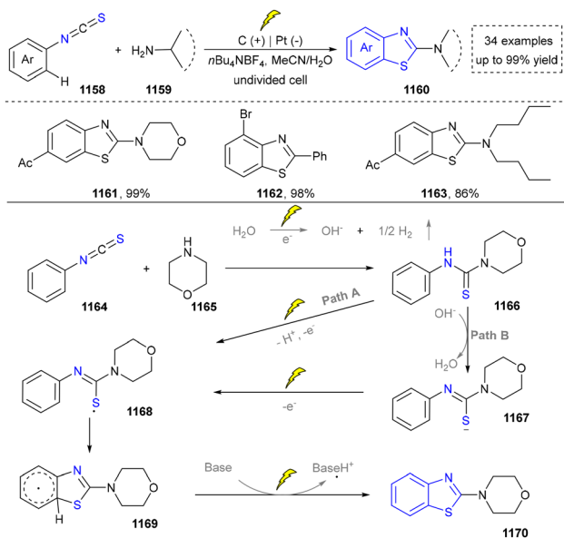
Scheme 123 Electrochemical dehydrogenation for the synthesis of benzothiazoles.
