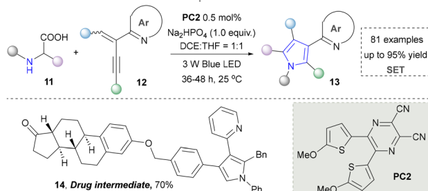
Scheme 2 Assembly of the azaarene-substituted pyrroles based on radical construction.
