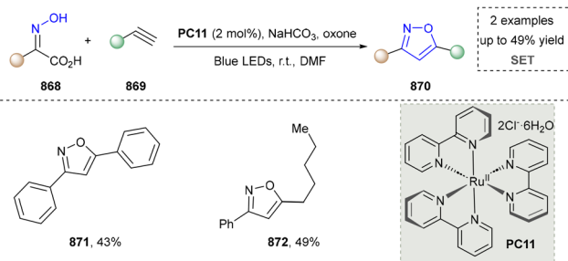
Scheme 92 Visible light promoted the synthesis of isoxazoles.
