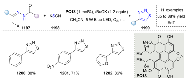
Scheme 126 Photocatalytic method to afford the 1,2,3-thiadiazole derivatives.
