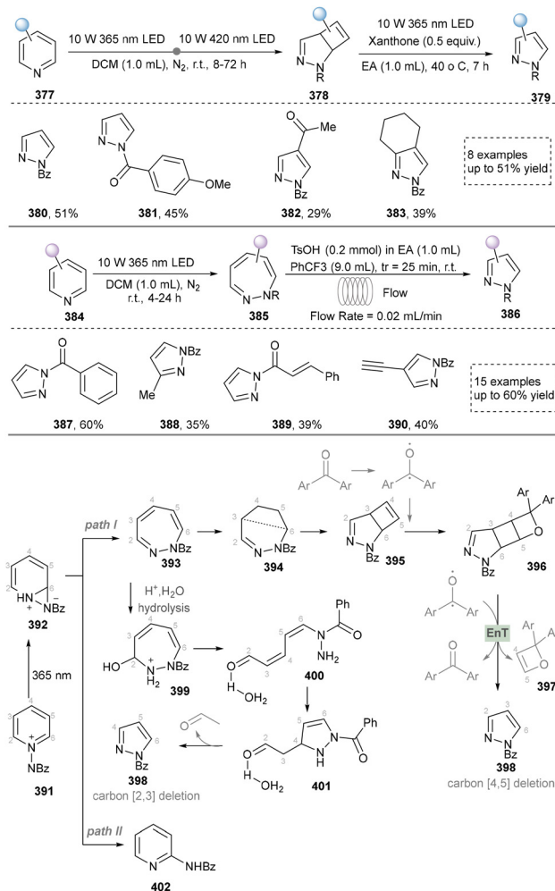
Scheme 42 Photochemical skeletal editing of pyridines to pyrazoles.
