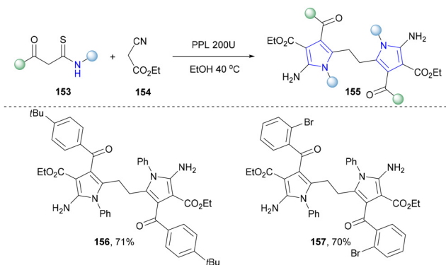
Scheme 15 Enzymatic synthesis of pyrrole disulfides by lipase.
