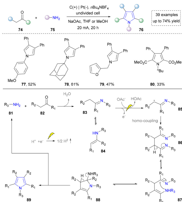
Scheme 8 Electrochemical oxidative annulation of amines and aldehydes/ketones for the synthesis of pyrroles.
