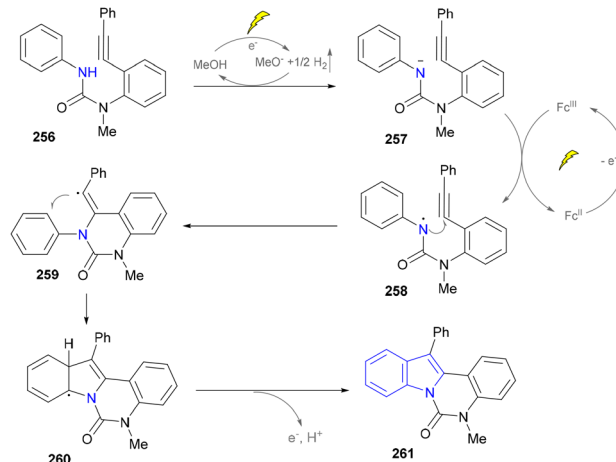
Scheme 27 (Aza)indole synthesis by C–H/N–H functionalization.
