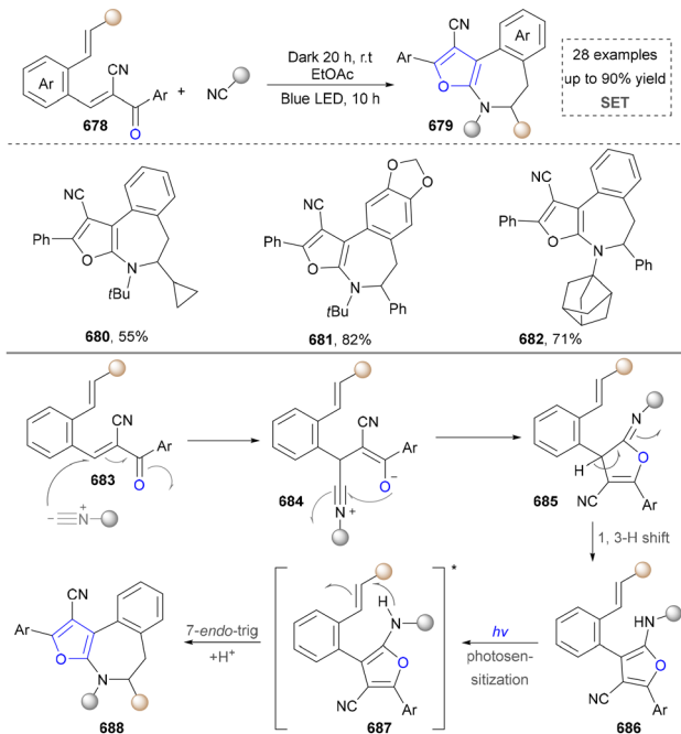
Scheme 73 Photocatalyst-free and transition-metal-free synthesis of furans.
