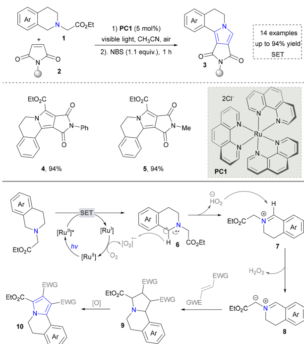
Scheme 1 Visible-light-induced oxidation/[3+2] cycloaddition/oxidative arylation sequence to obtain pyrroles.
