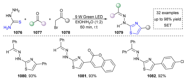
Scheme 114 Visible-light-induced synthesis of the 2-(2-hydrazinyl)thiazole derivatives.
