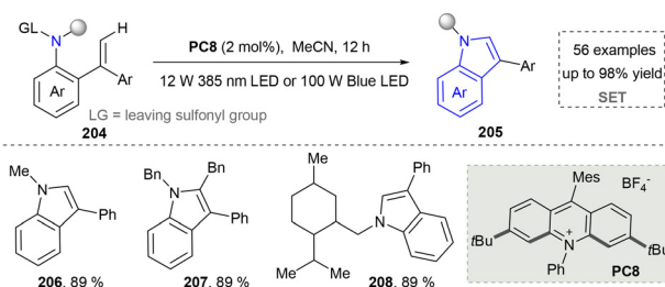
Scheme 21 Photoinduced synthesis of indoles via intramolecular C–N bond formation.
