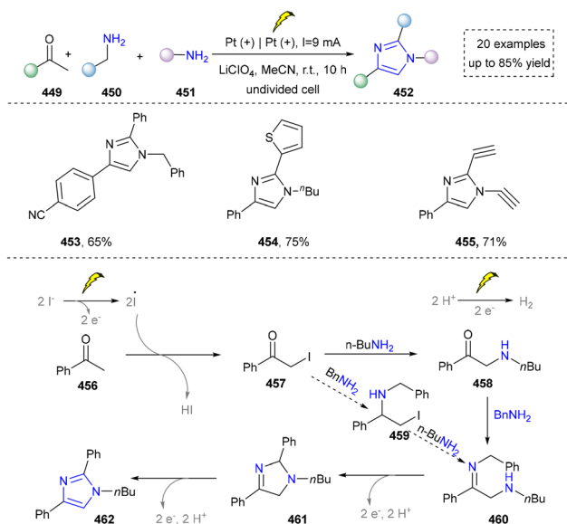
Scheme 48 Electrochemical oxidative annulation of ketones and amines used to produce imidazoles.
