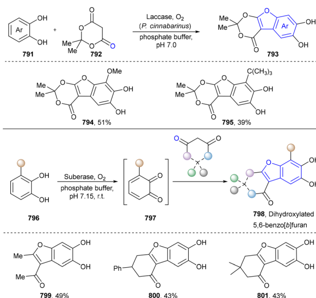
Scheme 84 Enzymatic synthesis of the benzofuran derivatives by laccase.
