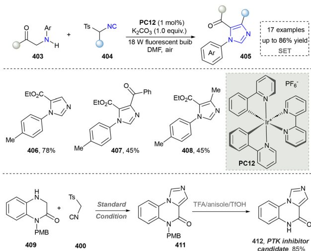
Scheme 43 Synthesis of imidazoles by photocatalytic aerobic oxidation/[3+2] cycloaddition.
