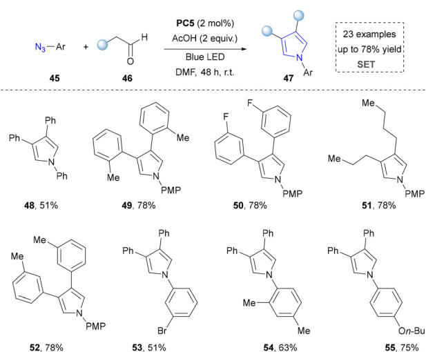
Scheme 6 Synthesis of 1,3,4-trisubstituted pyrroles from aryl azides.
