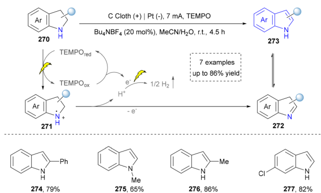
Scheme 29 TEMPO-promoted electrochemical receptor-free dehydrogenation of N-heterocycles.
