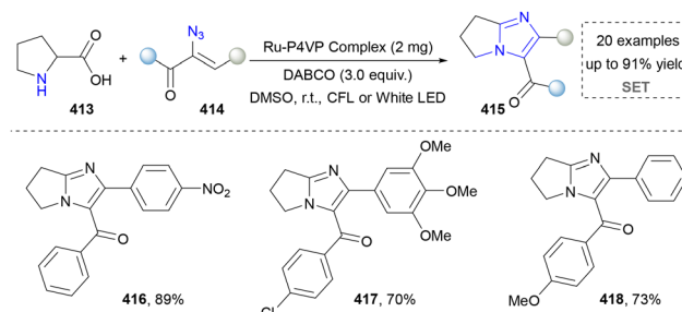
Scheme 44 Photo-induced decarboxylated annulative achieve imidazoles.
