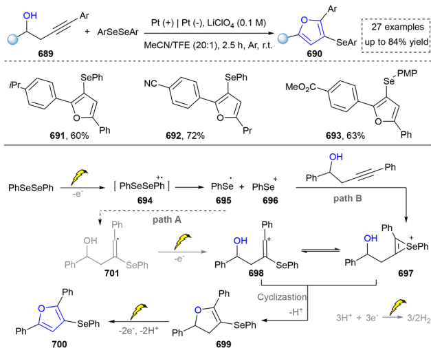
Scheme 74 Synthesis of polysubstituted furans through electrochemical selenocyclization.
