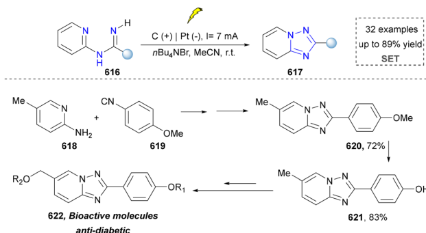
Scheme 66 Synthesis of 1,2,4-triazoles via intramolecular electrochemical dehydrogenation.
