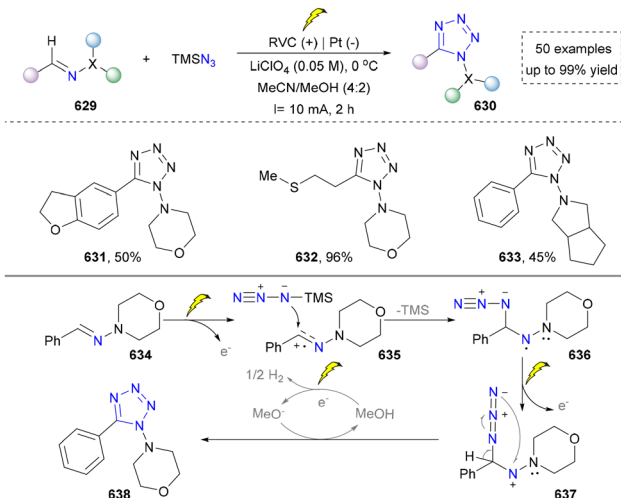
Scheme 68 Electrochemical synthesis of tetrazoles via the [3+2] cycloaddition of azides with hydrazones.
