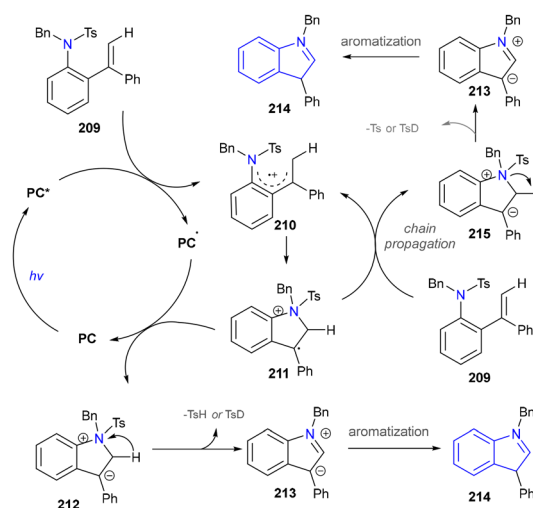
Scheme 22 Mechanism of the visible-light-induced indole synthesis through intramolecular C–N bond formation.
