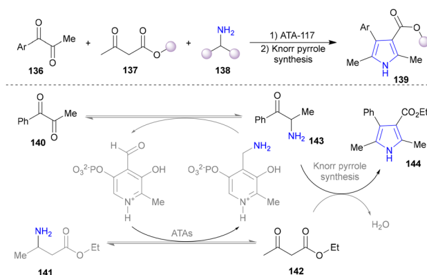
Scheme 13 Chemo-enzymatic cascades for the synthesis of pyrroles using ATA biocatalysts.
