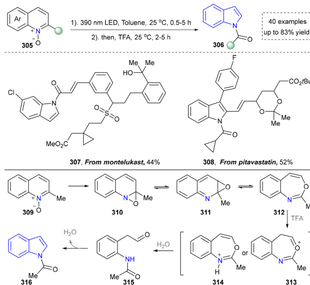
Scheme 34 Construction of indoles via photochemical skeletal editing.
