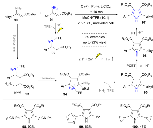
Scheme 9 Synthesis of the asymmetrically substituted NH-pyrroles by electrooxidation.
