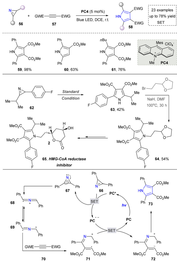
Scheme 7 Visible-light-induced [3+2] cycloaddition for the synthesis of pyrroles.
