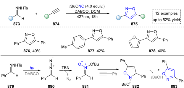
Scheme 93 Visible-light-mediated strategy for the synthesis of isoxazoles.
