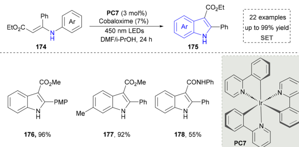
Scheme 18 Oxidant-free strategy for the synthesis of indoles under visible light irradiation.
