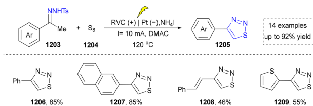
Scheme 127 Electrochemical synthesis of 1,2,3-thiadiazoles.
