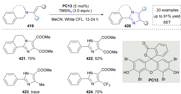
Scheme 45 Synthesis of imidazoles via dual C(sp 3 )-H and C(sp 2 )-H bond functionalization.
