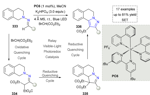
Scheme 37 Synthesis of the pyrazole derivatives via formal [4+1] annulation and aromatization.
