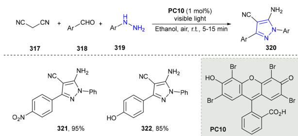
Scheme 35 Synthesis of pyrazoles from hydrazines under visible light irradiation.
