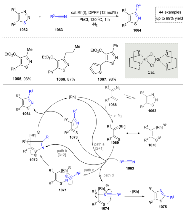
Scheme 113 Synthesis of isothiazoles via ring transformation of 1,2,3-thiadiazoles using nitriles.
