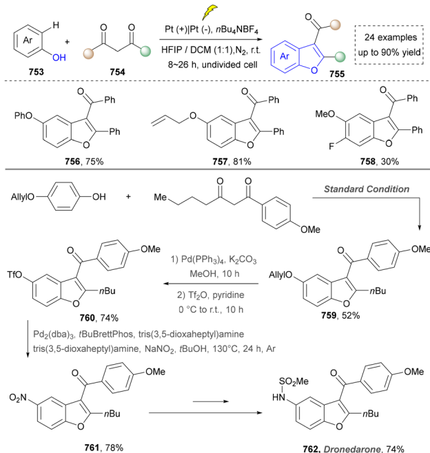
Scheme 81 Electrochemical cross-dehydrogenative coupling between phenols and \beta -dicarbonyl compounds.
