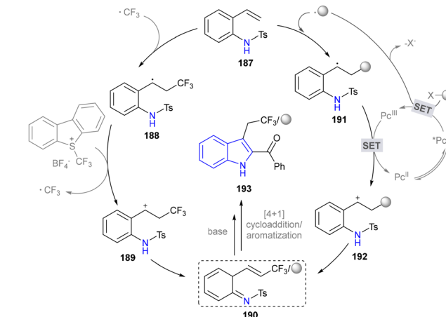
Scheme 19 Visible-light-driven aza- ortho -quinone methide generation.
