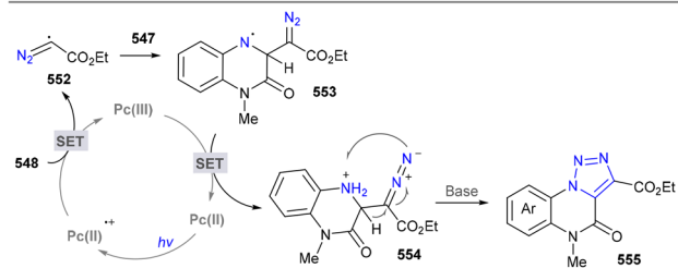
Scheme 57 Synthesis of 1,2,3-triazoles through photoredox-catalyzed [3+2] cyclization.
