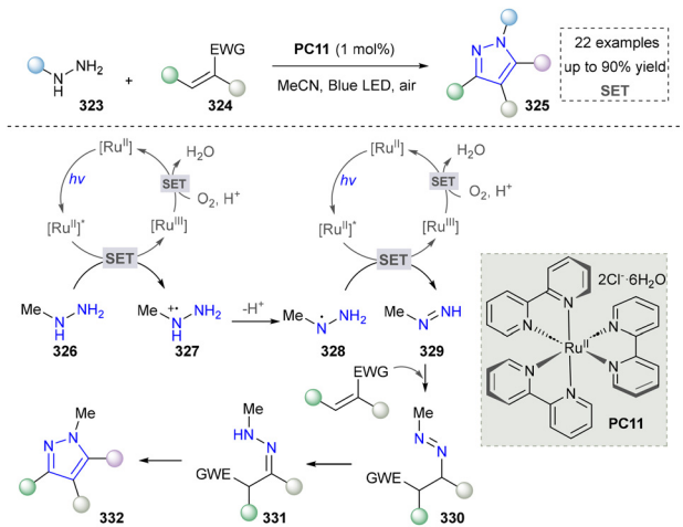
Scheme 36 Photocatalytic aerobic annulation for the green synthesis of pyrazoles.
