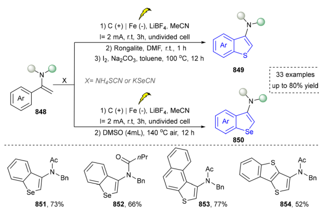
Scheme 90 Electrocatalytic synthesis of benzoselenophenes and benzothiophenes.
