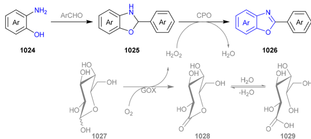
Scheme 109 Enzymatic synthesis of 2-substituted benzoxazoles via the GOX-CPO system.
