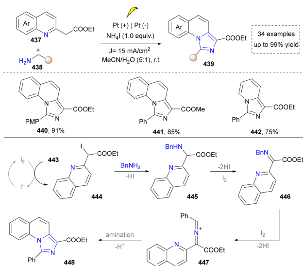
Scheme 47 Electrochemical synthesis of the 1,3-disubstituted imidazo[1,5- a ]quinolines.
