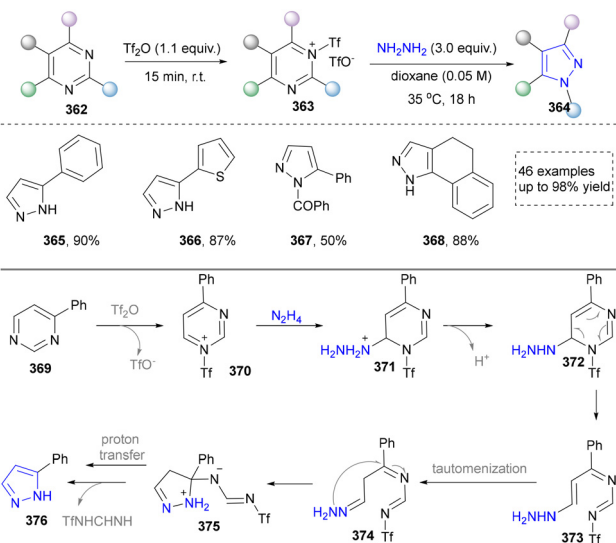
Scheme 41 Skeletal editing of pyrimidines to pyrazoles by formal carbon deletion.
