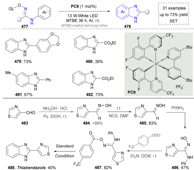
Scheme 51 N -Phenyl amidoxime esters to achieve the 2-substituted benzimidazoles.
