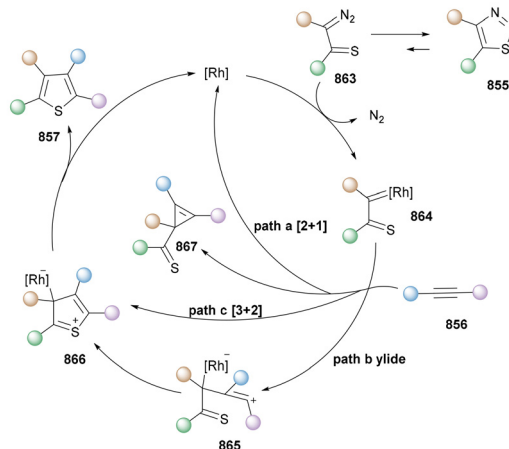
Scheme 91 Modular synthesis of polysubstituted thiophenes from 1,2,3-thiadiazoles.
