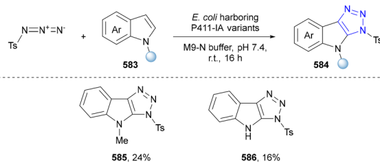
Scheme 62 Enzymatic synthesis of triazoles via indole-azide cycloaddition.
