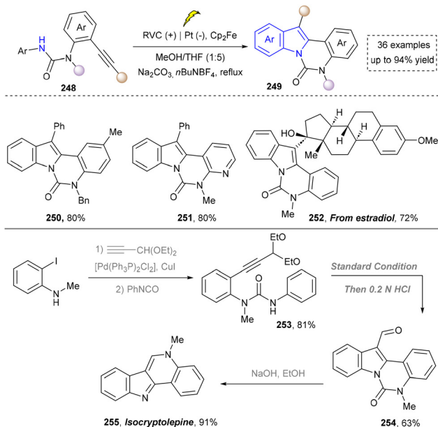
Scheme 26 Electrochemical C–H/N–H functionalization for the synthesis of indoles.
