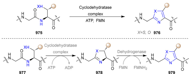
Scheme 103 Enzymatic synthesis of thiazole/oxazole-modified microcin.
