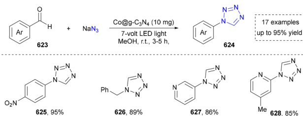
Scheme 67 Visible-light-driven synthesis of 1 H -tetrazoles through [3+2] cycloaddition.
