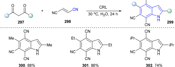
Scheme 32 Enzymatic synthesis of indoles utilizing lipase.
