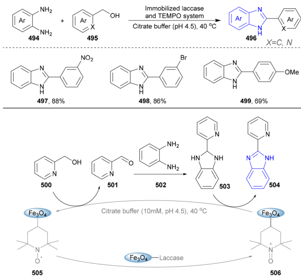
Scheme 53 Laccase-catalysed synthesis of benzimidazoles.
