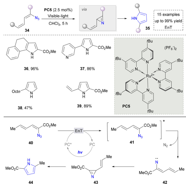
Scheme 5 The synthesis of pyrroles via visible light activation of aryl and vinyl azides.
