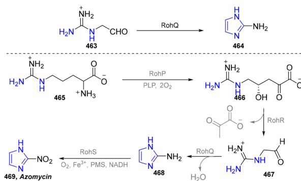
Scheme 49 Enzymatic synthesis of imidazoles from L-arginine.
