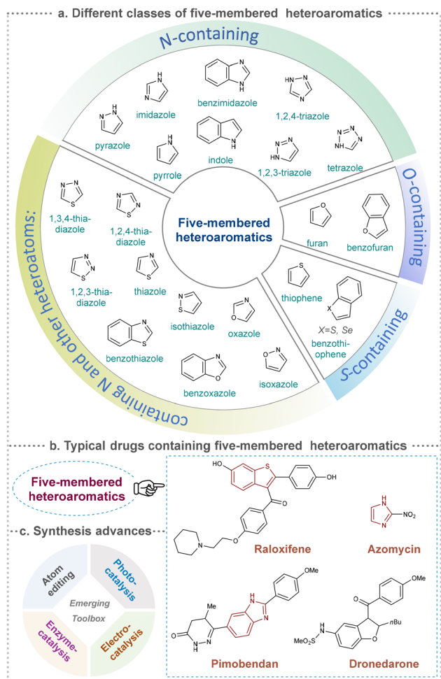
Fig. 1 Classification of different five-membered heteroaromatics and synthetic applications into drug molecules through emerging toolboxes.
