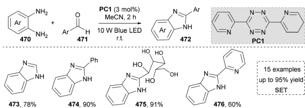
Scheme 50 Visible-light-driven green synthesis of the 2-substituted benzimidazoles.
