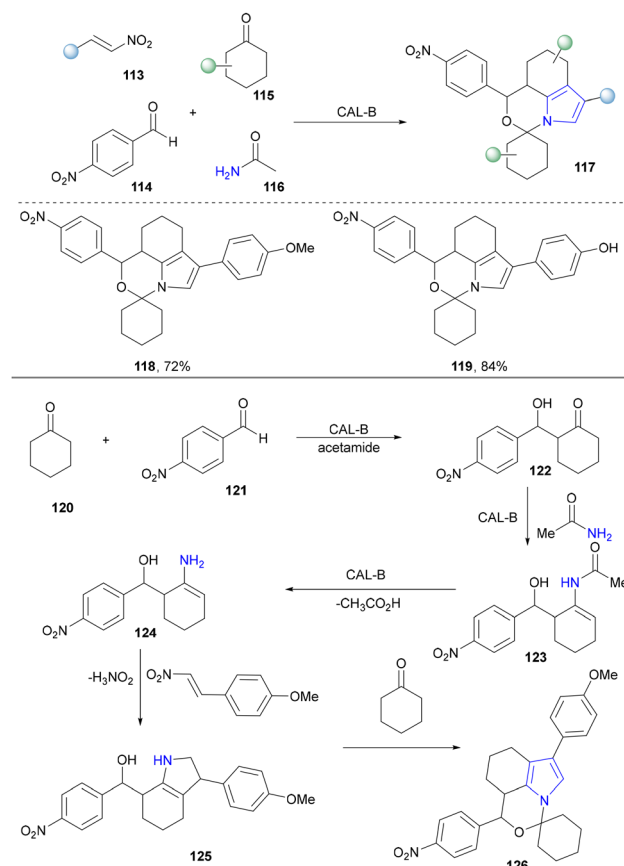
Scheme 11 Lipase-initiated synthesis of the spirooxazino derivatives.
