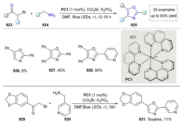
Scheme 97 Synthesis of substituted oxazoles by photocatalysis.
