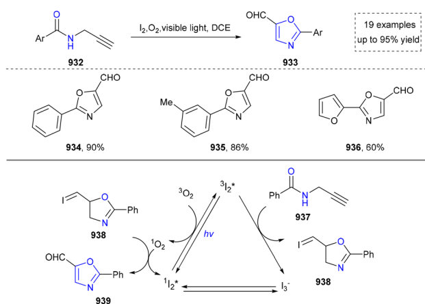
Scheme 98 Photocatalytic activation of alkynes for cyclization reactions.
