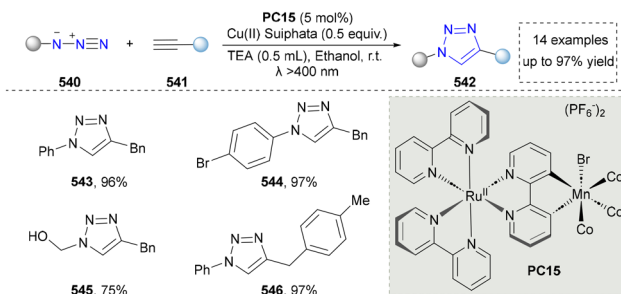
Scheme 56 Visible-light-assisted photocatalytic [3+2] reaction for the synthesis of 1,2,3-triazoles.
