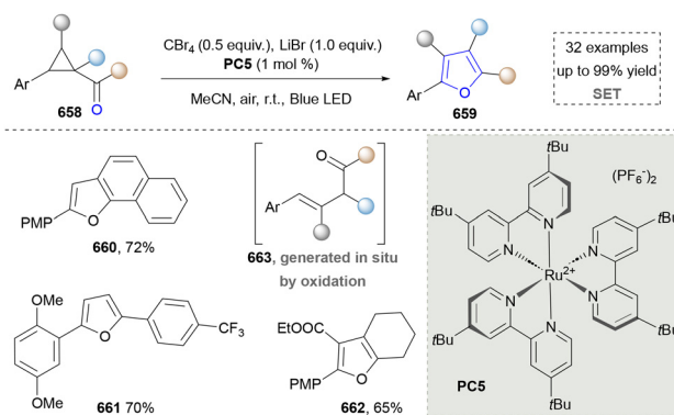
Scheme 71 Synthesis of polysubstituted furans from cyclopropyl ketones.
