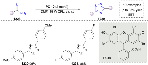
Scheme 129 Visible-light-driven aerobic oxidative cyclization to afford 1,2,4-thiadiazoles.
