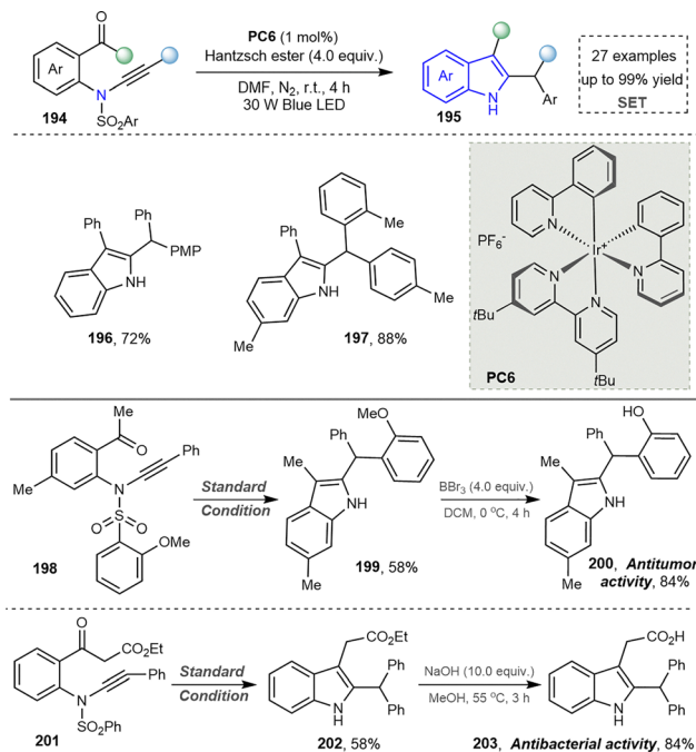
Scheme 20 Synthesis of the functionalized indoles from the visible light-mediated keto-amide coupling.
