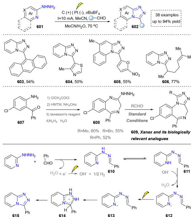
Scheme 65 Electrochemical synthesis of 1,2,4-triazole-fused heterocycles.
