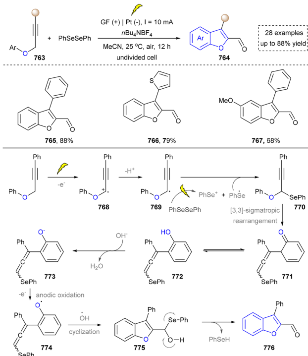
Scheme 82 Synthesis of benzofurans via an electrochemical cyclization reaction.
