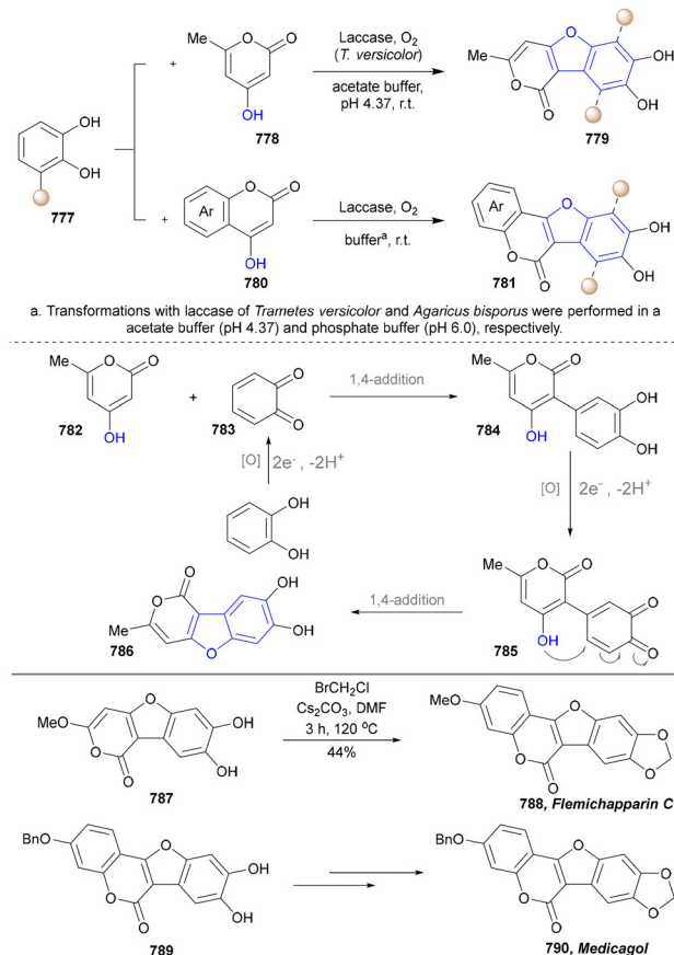
Scheme 83 Enzymatic synthesis of benzofurans by laccase.
