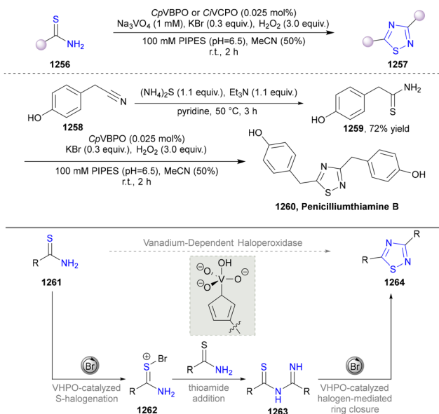
Scheme 132 1,2,4-Thiadiazole synthesis by vanadium-dependent haloperoxidases.
