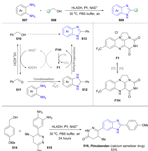
Scheme 54 Cooperative chemoenzymatic system for the synthesis of benzimidazoles.
