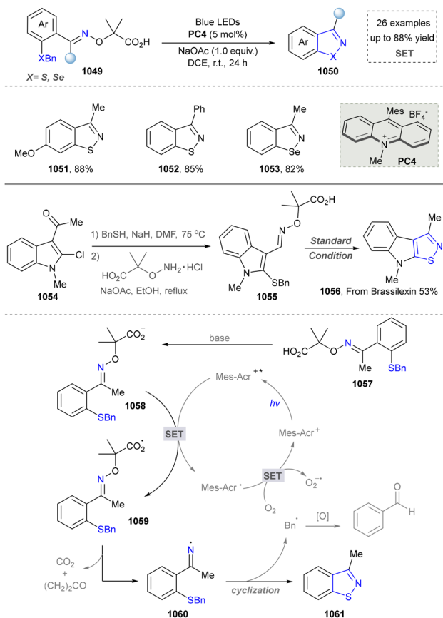
Scheme 112 Visible light-promoted N–S bond formation for the synthesis of isothiazoles.
