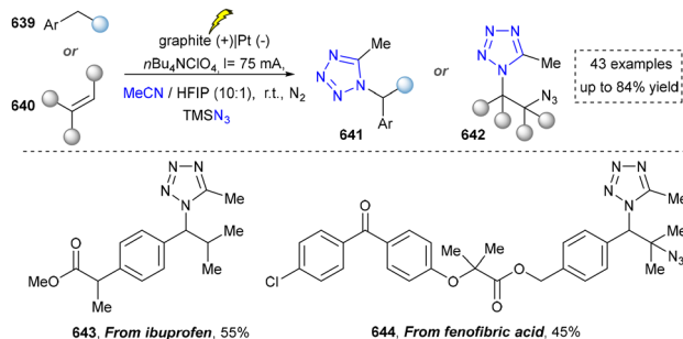
Scheme 69 Electrochemical multicomponent tetrazolization and vicinal azidotetrazolization.
