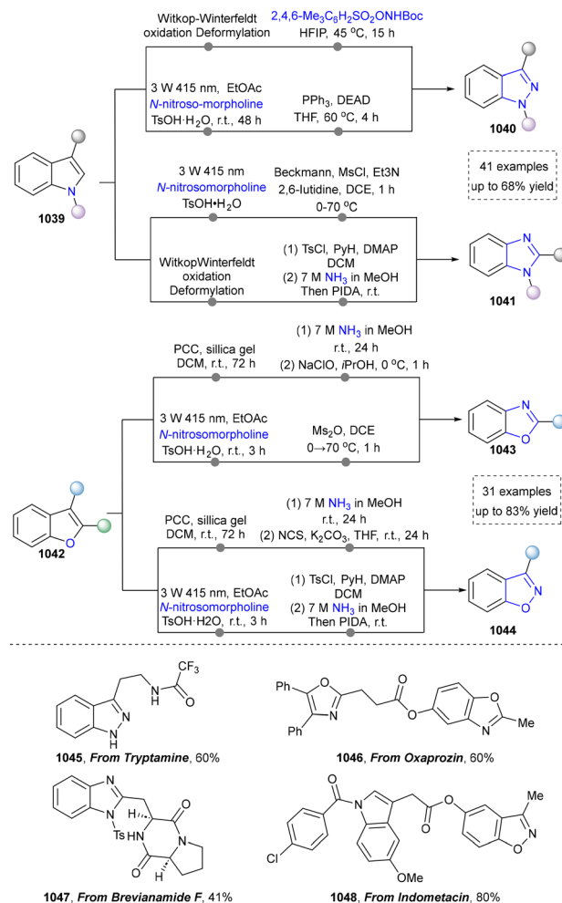
Scheme 111 Carbon-to-nitrogen atom exchange of indoles and benzofurans to form aromatic heterocycles.
