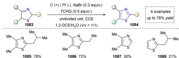
Scheme 115 Electrochemical synthesis of thiazoles.
