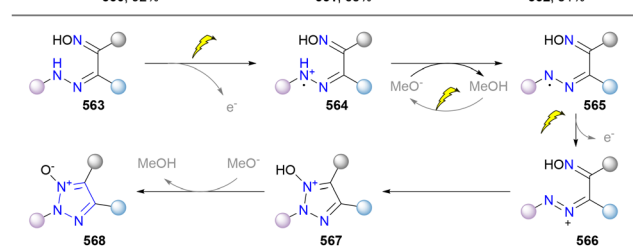
Scheme 59 Electrochemical N–N bond forming reactions: direct access to 1,2,3-triazoles.
