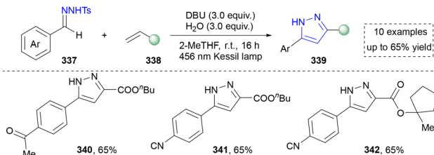
Scheme 38 Visible-light-induced [3+2] cycloadditions to achieve pyrazoles.
