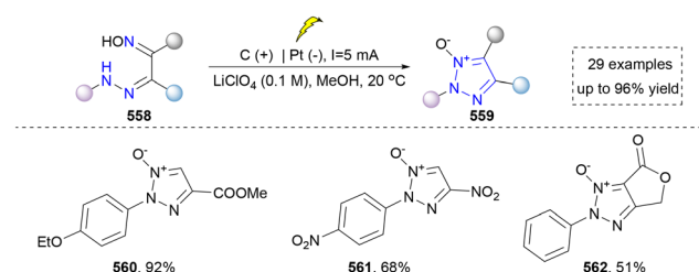
Scheme 58 Electrochemical synthesis of 1,2,3-triazole 1-oxides.
