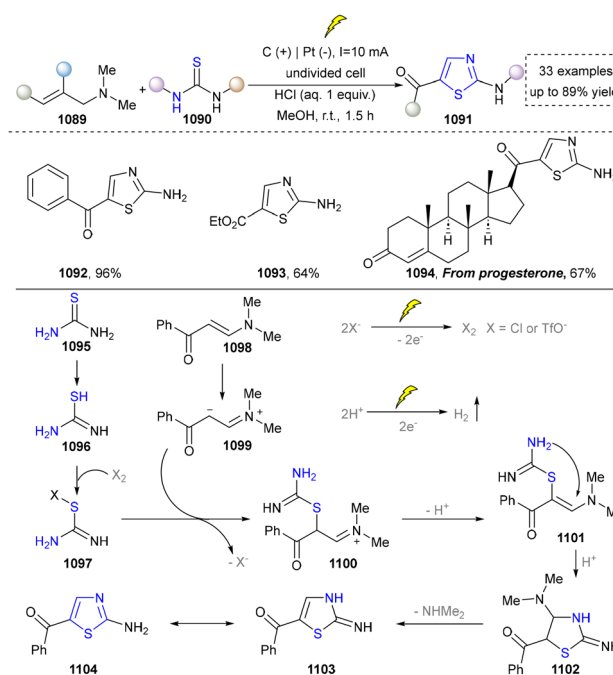
Scheme 116 Electrochemical C–H thiolation/C–N amination for thiazole synthesis.
