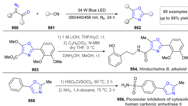
Scheme 100 Photoinduced [3+2] cycloaddition for the synthesis of oxazoles.
