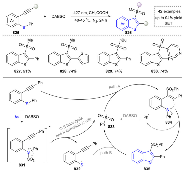
Scheme 88 Photo-induced synthesis of 3-(alkyl/arylsulfonyl) benzothiophenes.
