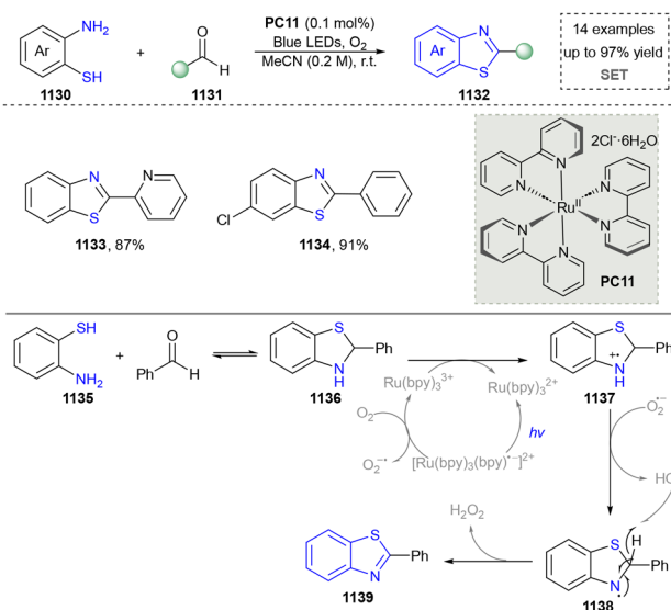
Scheme 120 Synthesis of the 2-substituted benzothiazoles via visible light-driven photoredox.
