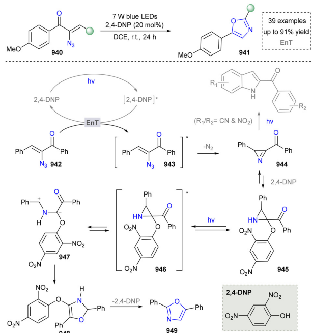
Scheme 99 Visible light promoted the conversion of \alpha -azidochalcones into 2,5-diaryloxazoles.
