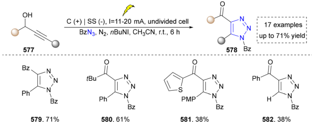
Scheme 61 Electrochemical synthesis of the novel N -benzoyl-1,2,3-triazole derivatives.
