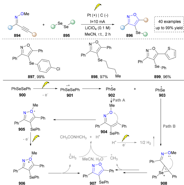
Scheme 95 Electrochemically promoted synthesis of organoselenenyl isoxazoles.
