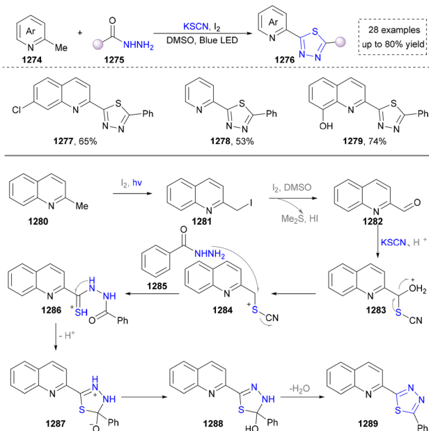
Scheme 134 Photoinduced construction of thiadiazole derivatives.
