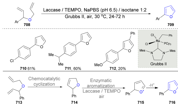
Scheme 76 Enzymatic synthesis of furans by T. versicolor laccase.
