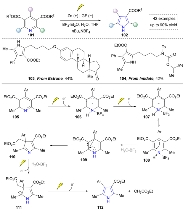
Scheme 10 Electrochemical strategy for the generation of pyrroles by ring contraction.
