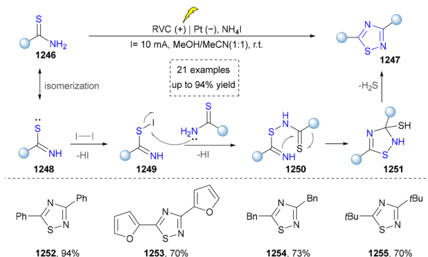
Scheme 131 Electrochemical synthesis of 3,5-disubstituted-1,2,4-thiadiazoles.
