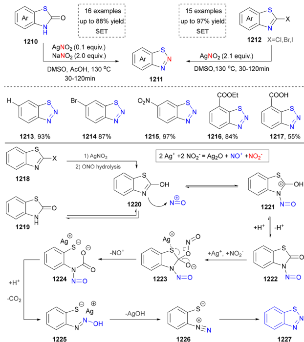
Scheme 128 Benzo[1,2,3]thiadiazole synthesis from benzothiazol-2(3H)-ones and 2-halobenzothiazoles by single-step skeletal editing.
