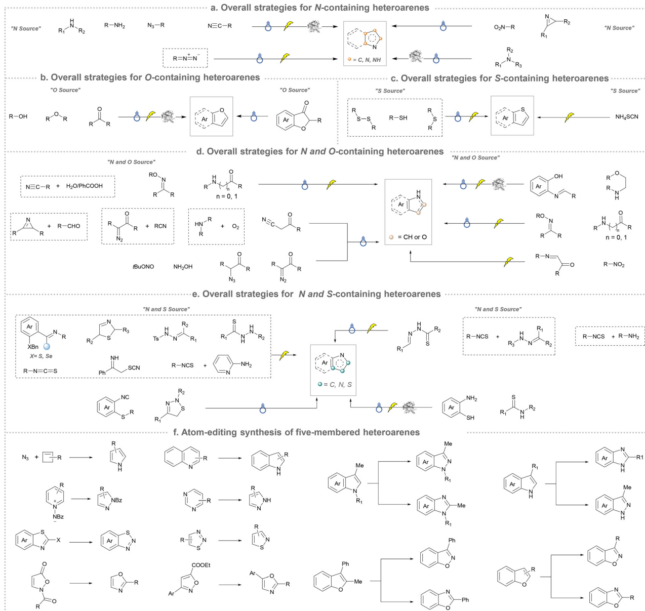
Fig. 2 Conceptual overview of synthesizing five-membered heteroaromatics via an emerging toolbox: (a) overall strategies for N-containing heteroarenes; (b) overall strategies for O-containing heteroarenes; (c) overall strategies for S-containing heteroarenes; (d) overall strategies for N and O-containing heteroarenes; (e) overall strategies for N and S-containing heteroarenes; (f) atom-editing synthesis of five-membered heteroarenes.
