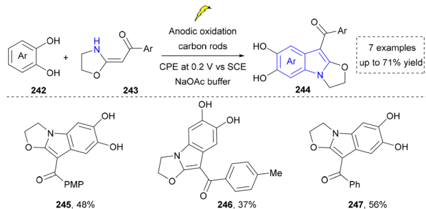
Scheme 25 Electrochemical synthesis of the fused indole derivatives.
