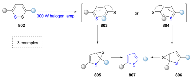
Scheme 85 Photoinduced synthesis of thiophenes.
