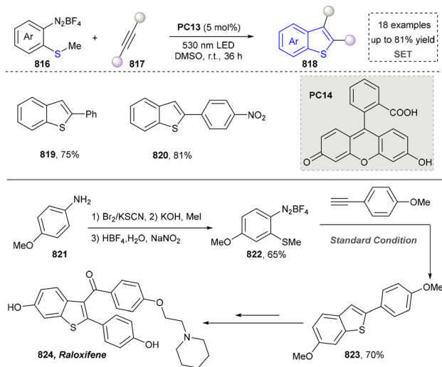
Scheme 87 Photocatalytic synthesis of benzothiophenes.
