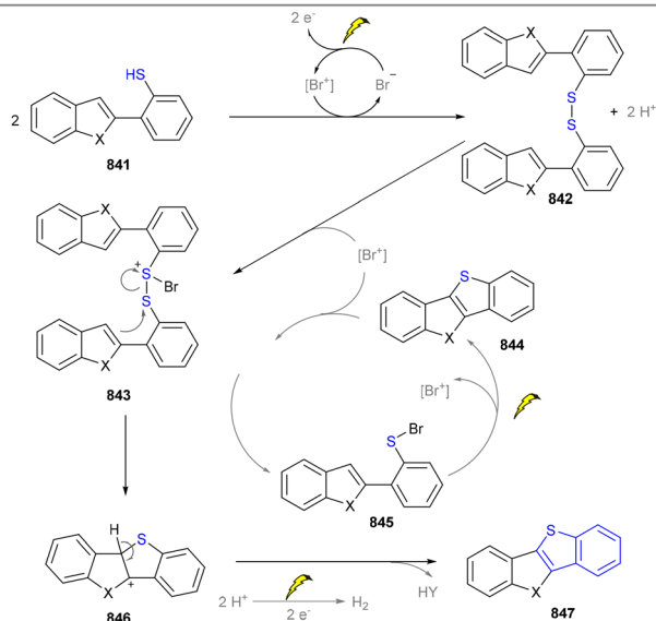
Scheme 89 Electrochemical synthesis of the thienoacene derivatives.
