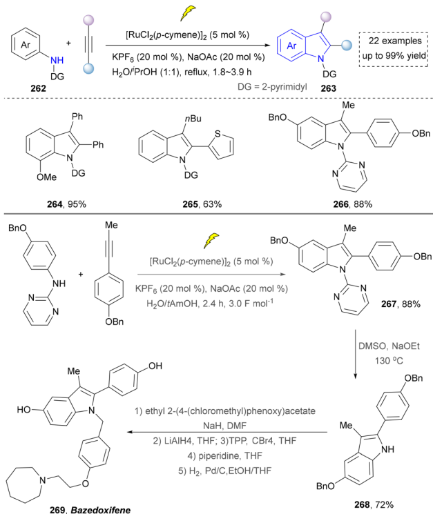
Scheme 28 Ruthenium-catalyzed electrochemical dehydrogenative alkyne annulation.
