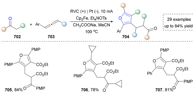
Scheme 75 Electrochemically-mediated C–H functionalization to construct furans.
