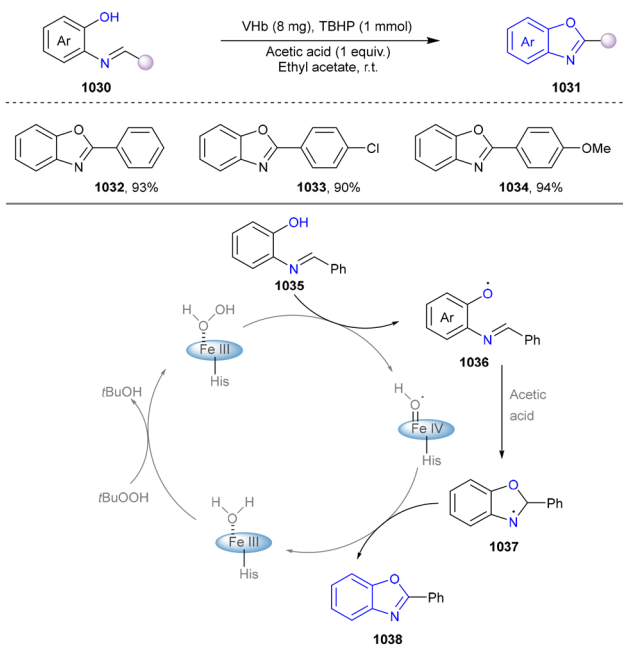
Scheme 110 Enzymatic synthesis of 2-substituted benzoxazoles via oxidative cyclization.
