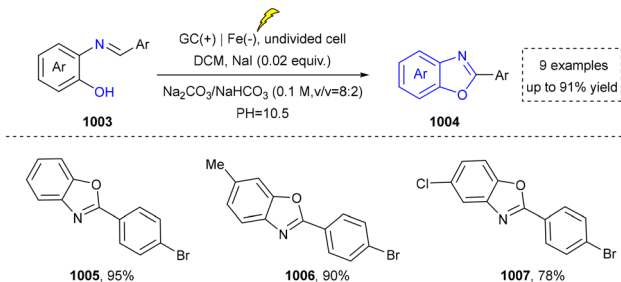
Scheme 106 Electrochemical synthesis of the 2-substituted benzoxazoles.
