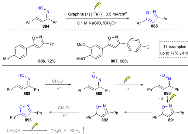
Scheme 94 Electrochemical synthesis of the 3,5-disubstituted isoxazoles.
