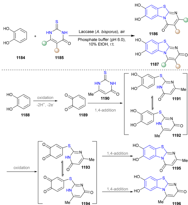
Scheme 125 Laccase-catalysed synthesis of pyrimidobenzothiazoles.
