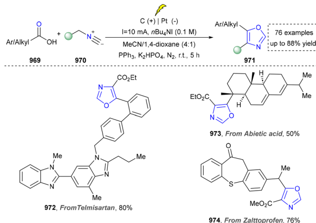
Scheme 102 Electrochemical synthesis of oxazoles via [3+2] cycloaddition.
