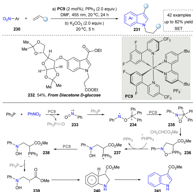
Scheme 24 Photocatalytic PPh 3 -mediated synthesis of C3-functionalized indoles.
