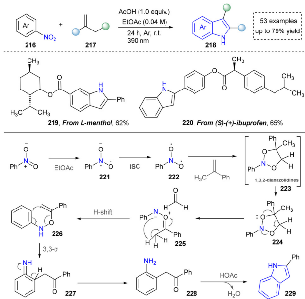
Scheme 23 Photoinduced Bartoli indole synthesis.
