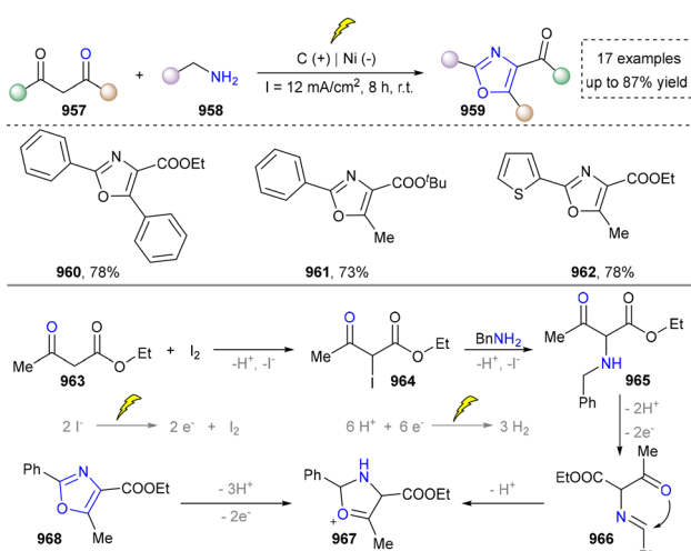
Scheme 101 Electrochemically promoted synthesis of polysubstituted oxazoles.
