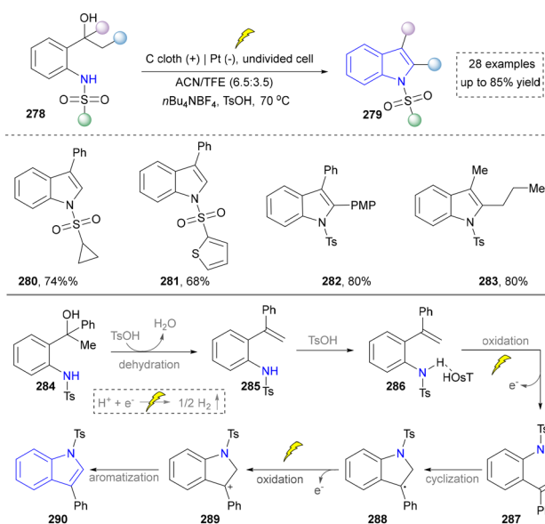
Scheme 30 Electrosynthesis of the substituted indoles from 1-(2-aminophenyl) alcohols.
