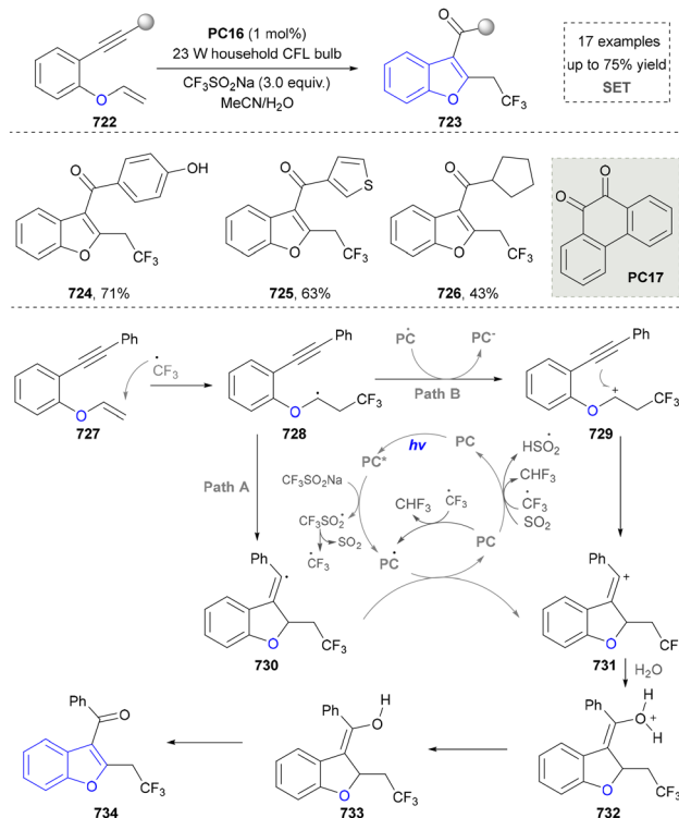
Scheme 78 Dehydrogenative cascade trifluoromethylation and oxidation.
