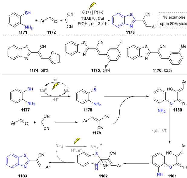
Scheme 124 Cu-catalyzed electron-relayed synthesis of 2-alkenylbenzothiazoles.
