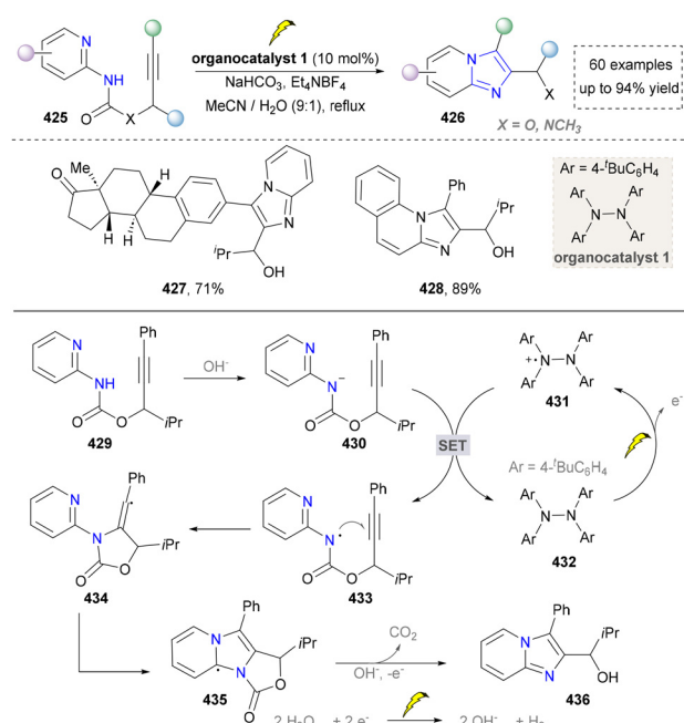
Scheme 46 Electrochemical synthesis of imidazoles through C-N bond formation.
