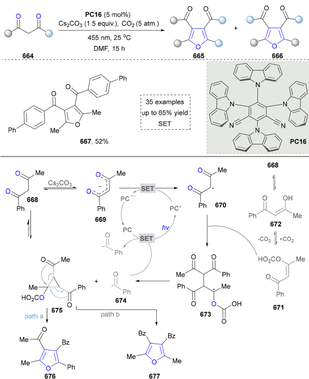
Scheme 72 Photocatalytic synthesis of furans promoted by carbon dioxide.
