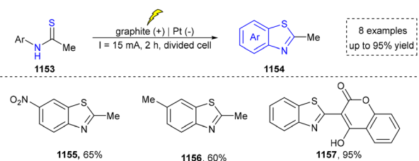
Scheme 122 Electrochemical synthesis of benzothiazole derivatives.
