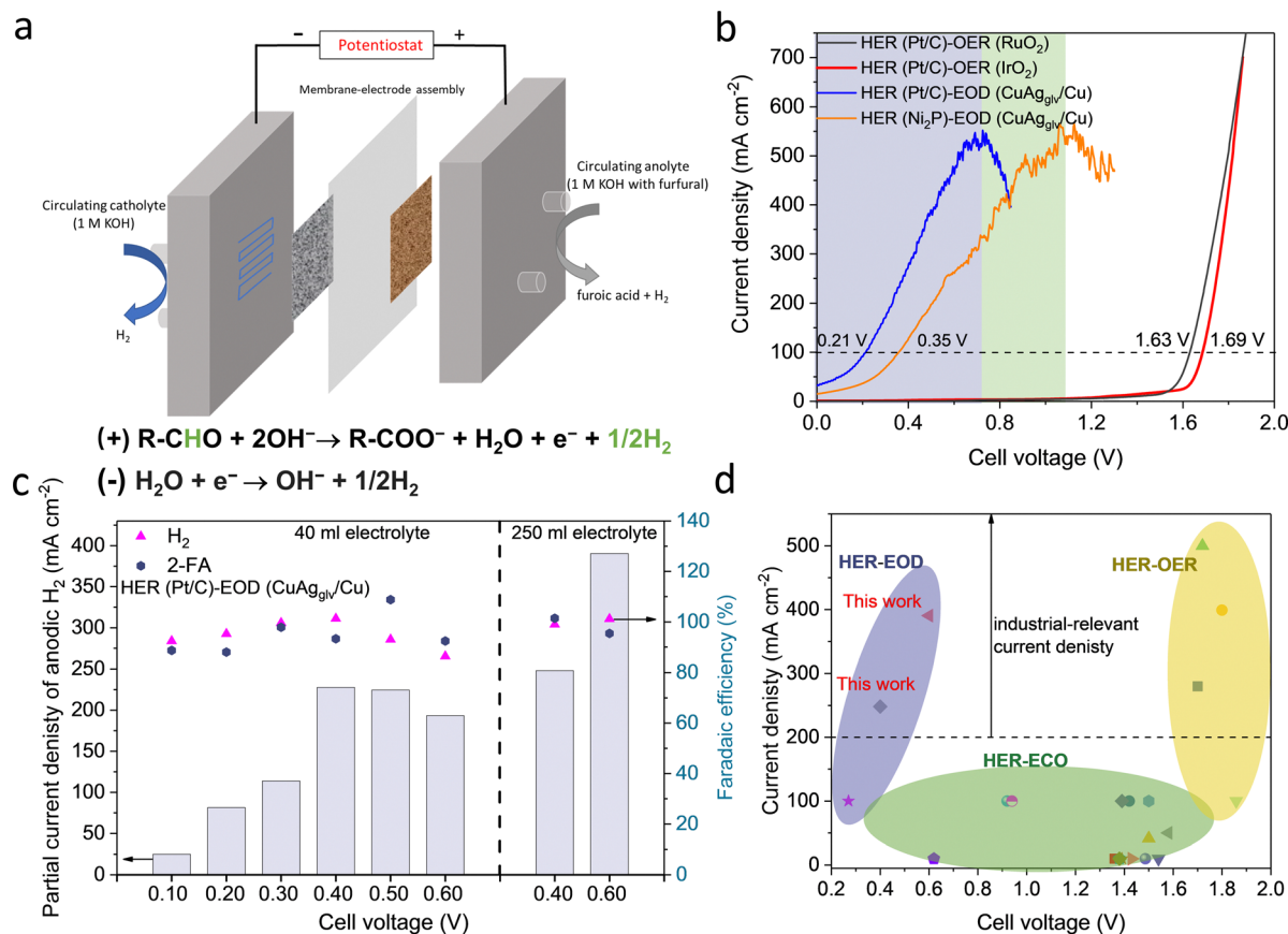
Fig. 5 Bipolar H_2 production in the MEA-based flow cells. (a) Scheme of the flow cell set-up and the reaction equations of bipolar H_2 production. The geometric area of anode was 1\text{ cm}^2 . (b) Linear sweep voltammograms for different paired reactions on different electrodes. (c) Partial current density of H_2 at different cell voltages with 40 ml and 250 ml of the electrolyte. The HER and EOD reaction were conducted on Pt/C and CuAg_{glv}/Cu , respectively. (d) Comparison of the performance of bipolar H_2 production in this work with previous works for electrochemical H_2 production, including HER-ECO paired H_2 production, and HER-OER paired water electrolysis.
