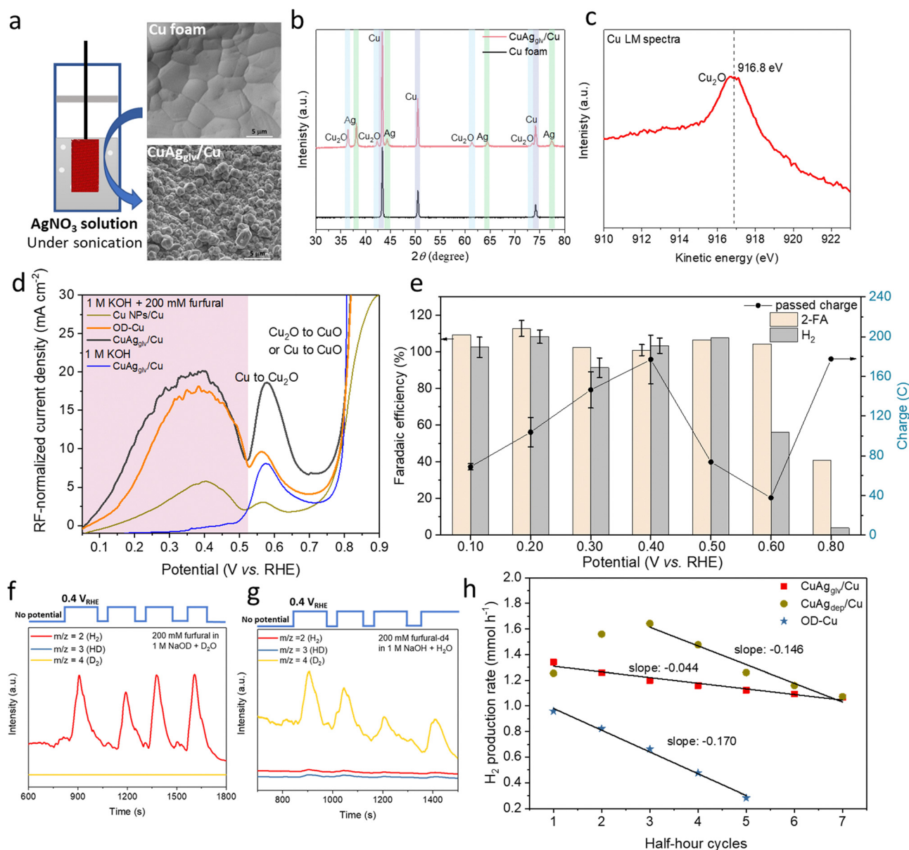
Fig. 3 EOD reaction on CuAg_{glv}/Cu in the H-type cell. (a) Scheme of the galvanic replacement method and SEM images of Cu foam and as-synthesized CuAg_{glv}/Cu . (b) XRD patterns of Cu foam and as-synthesized CuAg_{glv}/Cu . (c) Auger Cu LM spectrum of as-synthesized CuAg_{glv}/Cu . (d) Linear sweep voltammetry (2nd cycle) on Cu-based electrodes, including Cu NPs/Cu, OD-Cu, CuAg_{glv}/Cu , with or without 200 mM furfural in the 1 M KOH electrolyte. The current density was normalized to the roughness factor (RF). (e) Faradaic efficiency (left y-axis) and passed charge (right y-axis) in 1 M KOH with 200 mM furfural at different applied potentials on CuAg_{glv}/Cu for half-hour electrolysis. The geometric area for the electrode was 1\text{ cm}^2 . (f) and (g) DEMS signals at m/z = 2, 3 , and 4 at a pulsed potential of 0.4\text{ V}_{RHE} on the CuAg_{glv}/Cu electrode. Measurements in two deuterated electrolytes were performed: (f) 200 mM furfural in D_2O with 1 M NaOD and (g) furfural- d_4 in H_2O with 1 M NaOH. (h) H_2 production rate at different numbers of cycle for independent half-hour electrolysis with different Cu-based electrodes: OD-Cu, CuAg_{glv}/Cu , and CuAg_{dep}/Cu . A fresh electrolyte was replaced after each half-hour electrolysis. The slopes in (h) show their degradation rate.
