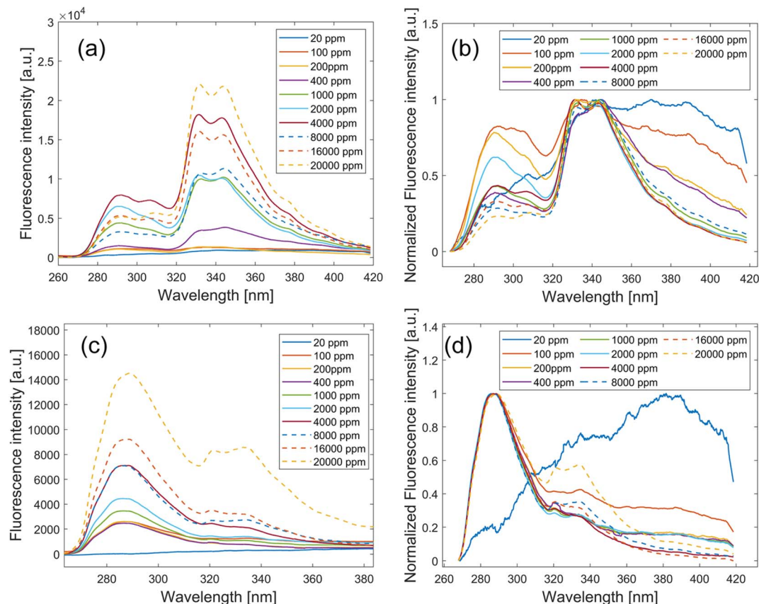
Fig. 5 Fluorescence spectra of -35# D and 95# G for different emulsion concentrations. (a) Initial fluorescence spectra of -35# D. (b) Normalized fluorescence spectra of -35# D. (c) Initial fluorescence spectra of 95# G. (d) Normalized fluorescence spectra of 95# G.
