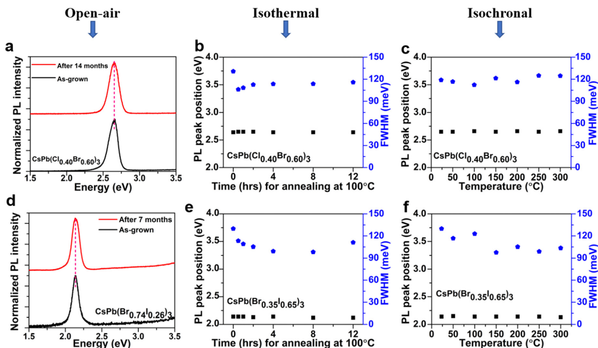
Fig. 5 Stability of quaternary halide perovskite alloy microplates. (a) and (d) Room-temperature ambient-air stability over a period of 14 and 7 months respectively for \text{CsPb}(\text{Cl}_{0.4}\text{Br}_{0.6})_3 and \text{CsPb}(\text{Br}_{0.74}\text{I}_{0.26})_3 microplates. (b), (c) and (e), (f) Thermal stability of representative \text{CsPb}(\text{Cl}_{1-x}\text{Br}_x)_3 and \text{CsPb}(\text{Br}_{1-x}\text{I}_x)_3 alloy samples, respectively. PL measurements of microplates after (b) and (e) isothermal annealing at 100^\circ\text{C} for different time periods of 0–12 hours and (c) and (f) isochronal annealing for 300 s in the temperature range between 0 and 300^\circ\text{C} .
