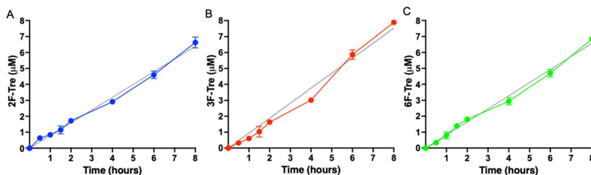
Fig. 6 Time dependent uptake of F-Tre analogues in Mycobacterium tuberculosis . Mtb was cultured in the presence of (A) 2F-Tre, (B) 3F-Tre and (C) 6F-Tre (100 \mu M) and the cytosolic extracts sampled at the time points indicated and analysed by high performance anion exchange chromatography with pulsed amperometric detection (HPAEC-PAD). Error bars denote the standard deviation from duplicate experiments. Simple linear regression fit is shown with a black dotted line (A) y = 80x ; (B) y = 0.94x ; (C) y = 0.82x . The concentration values are in Table S6.† Representative ion-chromatography traces are shown in Fig. S8† and retention times are in Table S7.†
