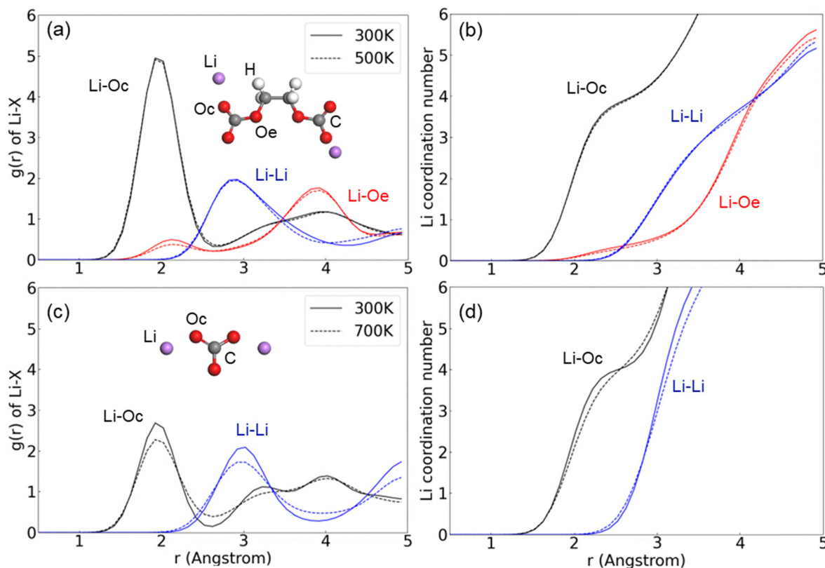
Fig. 8 Radial distribution functions (a) and (c) of Li-X (X = Oc, Oe and Li) and the coordination numbers of Li for Li-X (b) and (d) obtained from MD simulations of amorphous Li 2 EDC and crystalline Li 2 CO 3 at different temperatures.
