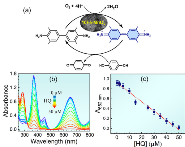
Fig. 9 (a) Schematic for TMB oxidation and subsequent detection of HQ; (b) UV-Vis spectra of the 10\text{Fe-MnO}_x /TMB system in the presence of various concentrations of HQ (0–50 \mu\text{M} ) and (c) calibration curve for the detection of HQ using 10\text{Fe-MnO}_x /TMB.
