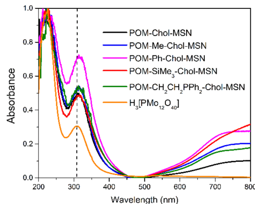
Fig. 4 DRUV-vis spectra of POM-based materials in comparison with that of H_3[PMo_{12}O_{40}] .
