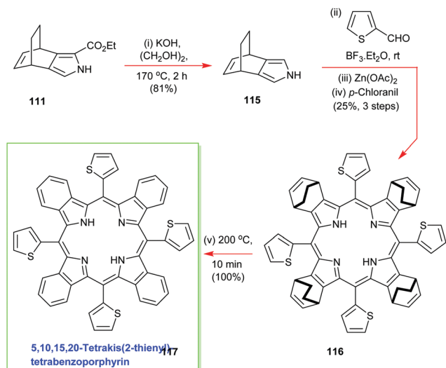
Scheme 16 Ono's masked-isoidole route to 5,10,15,20-tetrakis(2-thienyl)tetrabenzoporphyrin 117 .
