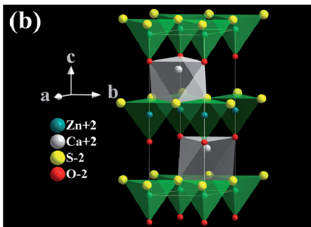
Fig. 3 (a) X-ray diffraction patterns of the as-prepared samples and the pattern of ICSID#245309 for CaZnOS; (b) crystal structure of CaZnOS.
