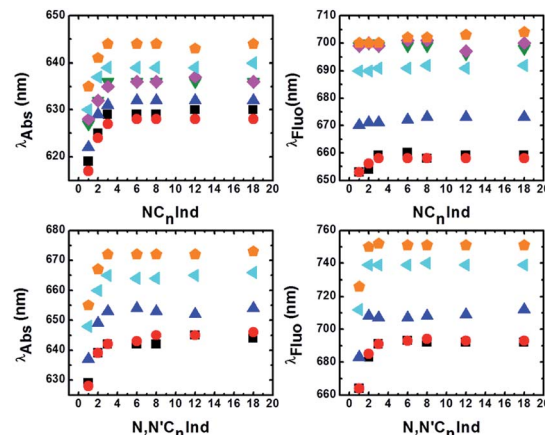
Fig. 2 Dependence of the spectroscopic properties (wavelength maxima of absorption, \lambda_{\text{Abs}} , and of fluorescence, \lambda_{\text{Fluo}} ) for the N -alkyl ( \text{NC}_n\text{Ind} ) and N,N' -dialkyl ( \text{N},\text{N}'\text{C}_n\text{Ind} ) indigo derivatives on n -dodecane (black squares), MCH (red circles), 2MeTHF (blue triangles), EtOH (green triangles), MeOH (pink rhombi), DMF (cyan triangles) and DMSO (orange pentagons) at T = 293 K.
