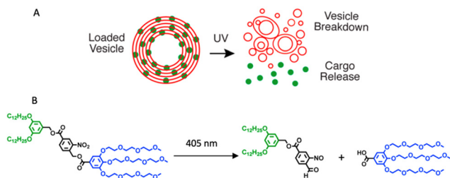
Fig. 4 A schematic showing the photocleavable dendrimersomes breakdown and cargo release upon UV irradiation (A). Photocleavage of amphiphilic Janus dendrimers containing a single ortho -nitrobenzyl unit between hydrophobic and hydrophilic dendrons (B). Reproduced from ref. 20 with permission of American Chemical Society.
