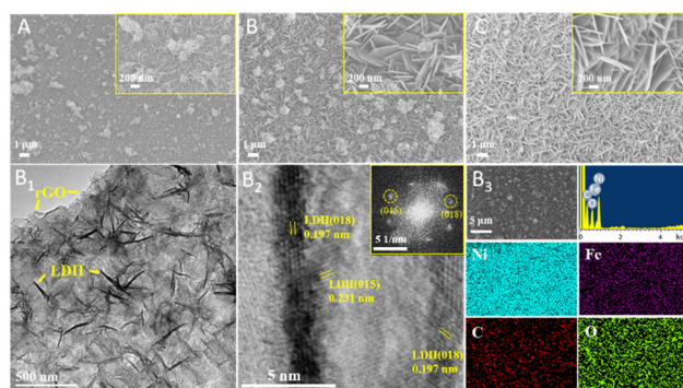
Fig. 2 SEM images of \text{Ni}_x\text{Fe}_{1-x}\text{LDH}/\text{rGO}/\text{NF} ( x = 3, 2, 1 ; A, B, C), and TEM ( B_1 ), HRTEM ( B_2 , inset: FFT), EDS and elemental mapping ( B_3 ) of \text{Ni}_2\text{Fe}_1\text{-LDH}/\text{rGO}/\text{NF} .
