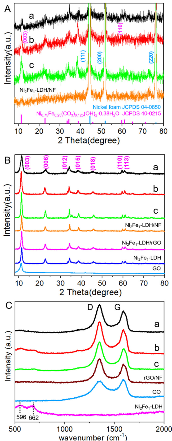
Fig. 1 XRD patterns (A and B) and Raman spectra (C) of the \text{Ni}_x\text{Fe}_{1-x}\text{LDH}/\text{rGO}/\text{NF} ( x = 3, 2, 1 ; a, b, c) composites (A and C) and the corresponding scraped powder samples (B) compared with those of \text{Ni}_2\text{Fe}_1\text{-LDH}/\text{NF} , \text{rGO}/\text{NF} , \text{GO} and \text{Ni}_2\text{Fe}_1\text{-LDH} .
