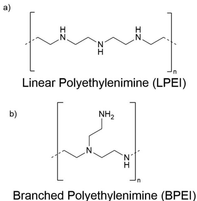
Fig. 1 Panels (a) and (b) represent the chemical structures of the polymer systems used in this study.
