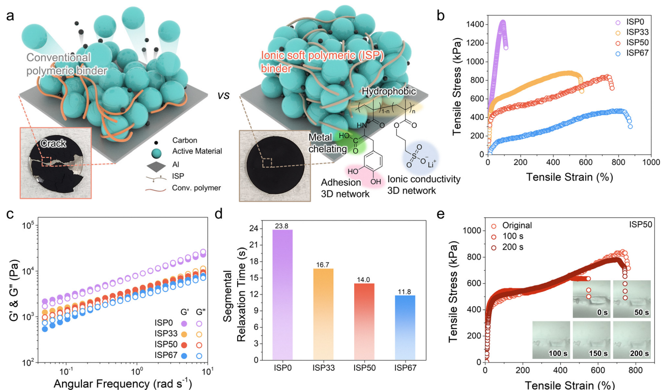
Fig. 1 (a) Illustration of a cathode based on conventional and ISP binders, along with the insets of the optical images of the cathode. (b) The tensile stress-strain ( S-S ) curves, (c) the storage ( G' ) and loss ( G'' ) moduli under angular frequencies, and the (d) segmental relaxation time ( \tau_s ) at 0.05 rad s -1 of the ISPs. (e) The tensile S-S curves depending on the time (quantitative self-healing), along with insets of optical microscopy (OM) images (qualitative self-healing) of the ISP50.
