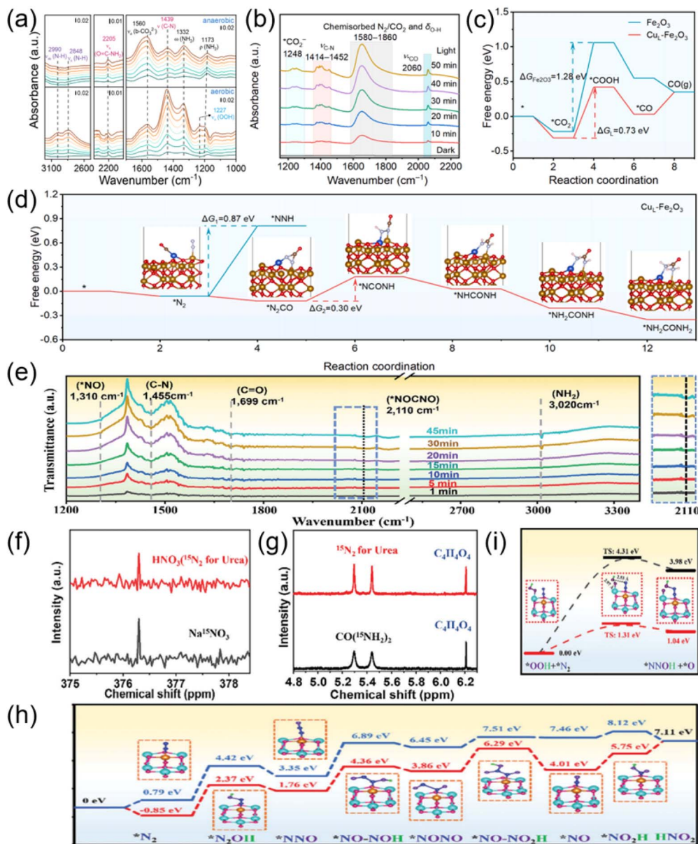
Fig. 3 (a) In situ FT-IR spectra of the photocatalytic urea synthesis under anaerobic (80% \text{CO} and 20% \text{Ar} ) or aerobic (80% \text{CO} and 20% \text{CO}_2 ) condition on \text{P25-4 h} . Reproduced with permission from ref. 46. Copyright 2025, Wiley-VCH. (b) In situ DRIFT of \text{Ni}_1\text{-CdS/WO}_3 during photocatalytic urea synthesis. Reproduced with permission from ref. 45. Copyright 2024, Wiley-VCH. (c) Gibbs free-energy profiles of the \text{CO}_2 reduction process for \text{Fe}_2\text{O}_3 and \text{CuL-Fe}_2\text{O}_3 . (d) Gibbs free-energy profiles and the geometric structure diagram of intermediates evolution during the urea synthesis process for \text{CuL-Fe}_2\text{O}_3 by alternating hydrogenation pathway. Reproduced with permission from ref. 37. Copyright 2025, Elsevier. (e) In situ ATR-FTIR spectroscopy measurements of \text{Ru-TiO}_2 over time during the coupling of \text{N}_2 and \text{CO}_2 . The enlargement at 2100\text{ cm}^{-1} is shown in blue on the right. (f) ^{15}\text{N} -NMR spectra of ^{15}\text{NO}_3^- (standard) and test product from NOR using ^{15}\text{N}_2 as feeding gas. (g) ^1\text{H} -NMR spectra of \text{CO}(^{15}\text{NH}_2)_2 (standard) and test product from urea using ^{15}\text{N}_2 as feeding gas. (h) Calculated free energy diagram for possible NOR mechanism on \text{TiO}_2 and \text{Ru-TiO}_2 (blue line: \text{TiO}_2 ; red line: \text{Ru-TiO}_2 ). (i) Reaction barrier diagrams from ^*\text{N}_2 to ^*\text{NNOH} on \text{TiO}_2 and \text{Ru-TiO}_2 (black line: \text{TiO}_2 ; red line: \text{Ru-TiO}_2 ). Reproduced with permission from ref. 48. Copyright 2024, Wiley-VCH.
