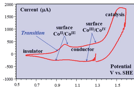
Fig. 5 Cyclic voltammetry current–potential responses (potential: 1.29 → 0.59 → 1.59 → 1.29 V vs. SHE) at 8 V s −1 of a 39 nm cobalt oxide deposited ( \text{CoP}_i ) film in the presence of 0.2 M potassium phosphate ( \text{KP}_i ) at pH = 7. Adapted from Fig. 2 in ref. 18 with permission.
