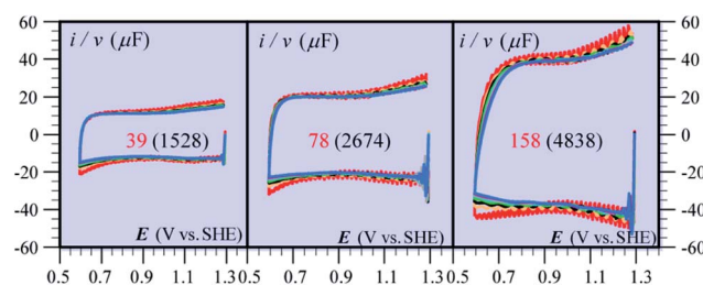
Fig. 6 Cyclic voltammetry current–potential responses at various scan rates ( \nu ) of \text{CoP}_i films at pH 7 in the presence of 1 mM \text{Pi} and 100 mM \text{KNO}_3 . \nu (V s −1 ): 1 (red), 2 (orange), 3 (black), 4 (green), 5 (cyan), 6 (gray), 7 (magenta), and 8 (blue). The numbers on each diagram are the values of film thickness in nm and, between parentheses, the value of the plateau capacitance in \mu\text{F cm}^{-2} . Adapted from ref. 18, with permission.
