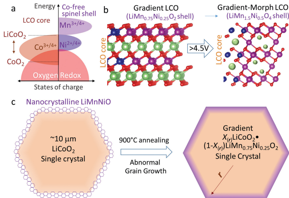
Fig. 1 Electronic bands, lattice structures and preparation process of \text{LiCoO}_2 and the gradient X(r)\text{LiCoO}_2 \cdot (1-X(r))\text{LiMn}_{0.75}\text{Ni}_{0.25}\text{O}_2 single-crystal. (a) The band structures in \text{LiCoO}_2 and Co-free LMO ( M = \text{Mn}, \text{Ni} etc.). (b) The surface reconstruction of the gradient X(r)\text{LiCoO}_2 \cdot (1-X(r))\text{LiMn}_{0.75}\text{Ni}_{0.25}\text{O}_2 crystal in the initial electrochemical formation. In this process, the oxygen sublattice maintains lattice-coherency during the layered \text{LiMn}_{0.75}\text{Ni}_{0.25}\text{O}_2 \rightarrow spinel \text{LiMn}_{1.5}\text{Ni}_{0.5}\text{O}_4 transformation, with preserved Mn : Ni : O ratio and no oxygen loss. The blue balls represent Co ions, while the violet, green and red balls represent Mn/Ni, Li and O ions, respectively. (c) Schematic showing the creation of the gradient X(r)\text{LiCoO}_2 \cdot (1-X(r))\text{LiMn}_{0.75}\text{Ni}_{0.25}\text{O}_2 single-crystal with an abnormal grain growth at high temperature.
