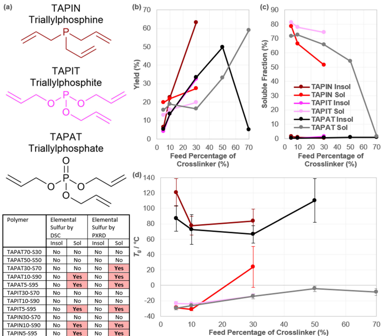
Fig. 7 (a) Chemical structures of TAPIN, TAPIT, and TAPAT as well as a table indicating whether elemental sulfur could be detected in the polymers by DSC or PXRD; (b) the yields of the Sol and Insol products at different weight percentages of crosslinker in the reaction feed for TAPIN, TAPIT, and TAPAT; (c) the soluble fractions of the Sol and Insol products at different weight percentages of crosslinker in the reaction feed for TAPIN, TAPIT, and TAPAT; (d) the T_g 's, obtained from the second heating cycle of DSC, of the Sol and Insol products at different weight percentages of crosslinker in the reaction feed for TAPIN, TAPIT, and TAPAT. Note that the error bars indicate the onset and end temperatures of the T_g . Where data points are missing, no T_g could be identified in the thermogram.
