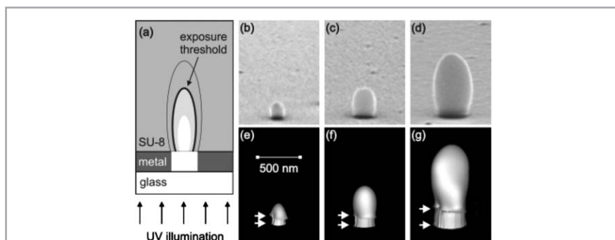
Fig. 67 Photolithographic mapping of light intensity transmission through an aluminium film. Panels (b)–(d) show the pattern in the SU-8 photoresist for hole diameters of 110, 200 and 360 nm. Panels (e)–(g) show the intensities calculated by the FDTD method. (Reprinted with permission from ref. 198. Copyright 2005, American Chemical Society.)
