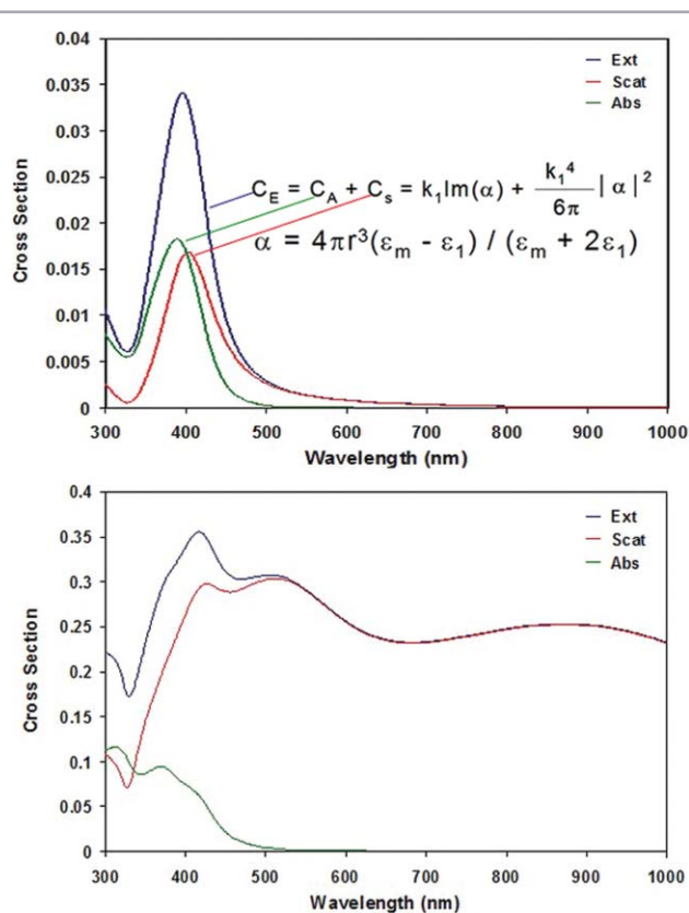
Fig. 7 Extinction, scattering and absorption cross-section of 80 nm Ag colloid (top) and 320 nm Ag colloid (bottom) calculated using Mie theory.
