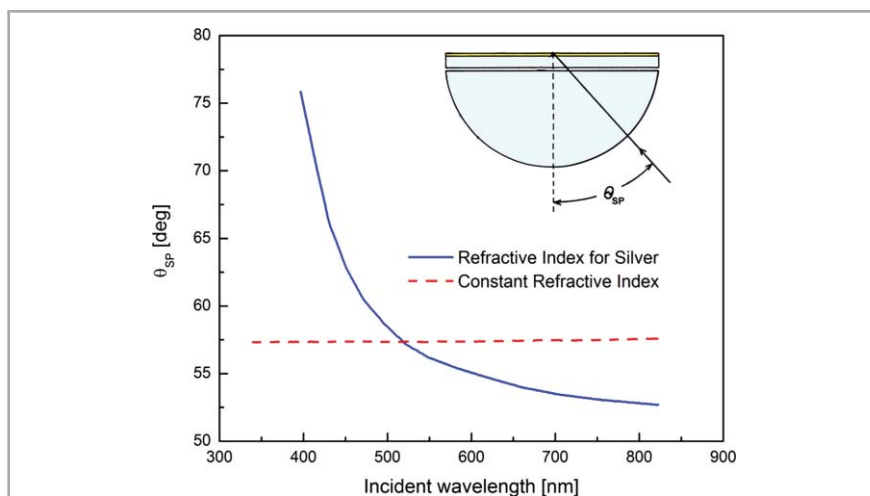
Fig. 42 Dependence of the surface plasmon angle \theta_{sp} on the incident wavelength for a real metal silver and for a material with a constant refractive index.
