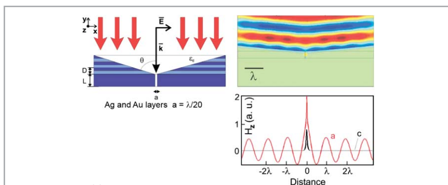
Fig. 68 Sub-wavelength excitation volumes using nano-apertures in layered metal films. (Reprinted with permission from ref. 199. Copyright 2006, Optical Society of America.)
