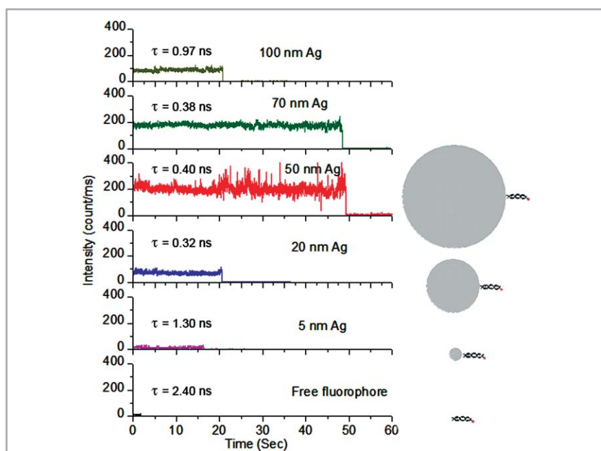
Fig. 21 Effects of silver particle size on single molecules of Cy5-DNA. Thiolated DNA was used to bind to the colloids. (Reprinted with permission from ref. 89. Copyright 2008, American Chemical Society.)
