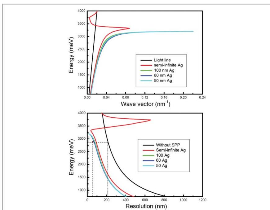
Fig. 69 Dispersion (top) and spatial resolution (bottom) of thin silver films. (Reprinted with permission from ref. 200. Copyright 2004, Optical Society of America.)
