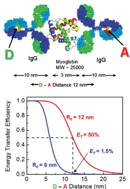
Fig. 25 Schematic of energy transfer in a sandwich assay with a change in R_0 . For this D–A pair the transfer efficiency is near 50% for the metal-enhanced R_0 = 12 nm and only 1.5% for R_0 = 6 nm without a metal particle.
