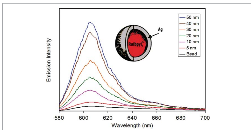
Fig. 27 Emission spectra of a silica bead containing \text{Ru}(\text{bpy})_3^{2+} alone and coated with an increasing thickness of a silver shell. (Reprinted with permission from ref. 105. Copyright 2006, American Chemical Society.)
