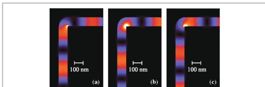
Fig. 57 FDTD simulations of plasmon transport in a slit in a metal film. The panels show the fields at t , t + 0.4 \times 10^{-15} s, and t + 0.8 \times 10^{-15} s. (Reprinted with permission from ref. 166. Copyright 2005, Optical Society of America.)
