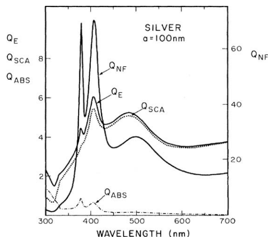
Fig. 9 Extinction, far-field scattering, and absorption efficiency (scale on the left side) compared with the near-field scattering efficiency (scale on the right side) for spheres with a = 100 nm immersed in water. (Reprinted with permission from ref. 41. Copyright 1981, American Physical Society.)
