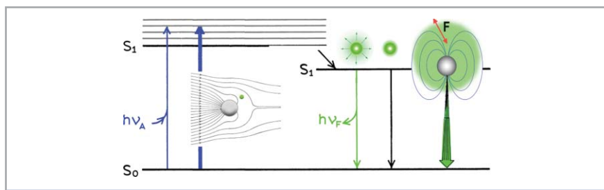
Fig. 3 Modified Jablonski diagram which includes metal–fluorophore interactions. The thicker arrows represent increased rates of excitation and emission.
