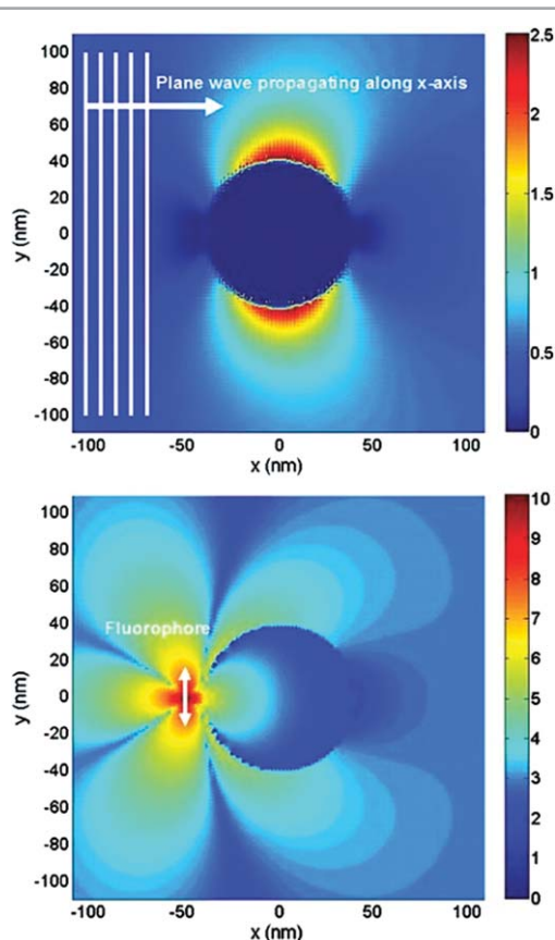
Fig. 11 Interaction of incident light with a colloid. Our FDTD calculations of the electric field around a 80 nm diameter silver colloid with 580 nm plane-wave illumination (top). Interaction of a 620 nm dipole fluorophore with a 80 nm colloid (bottom).
