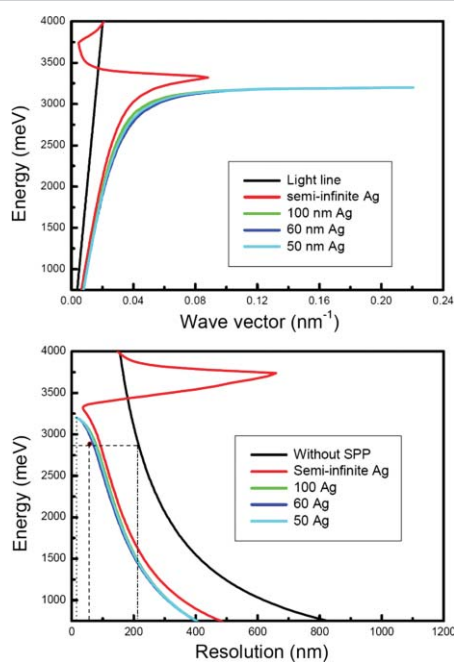
Fig. 69 Dispersion (top) and spatial resolution (bottom) of thin silver films. (Reprinted with permission from ref. 200. Copyright 2004, Optical Society of America.)
