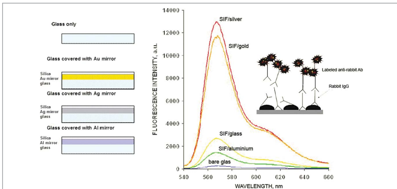
Fig. 47 Left: schematic of substrates with silver particles above a smooth metal film. Each substrate has silver particles on the silica. Right: emission spectra of Alexa Fluor 555 ® -labeled IgG on the substrates. (Reprinted with permission from ref. 143. Copyright 2007, Elsevier.)
