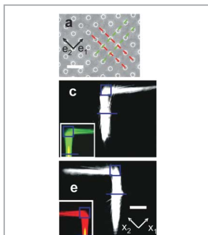
Fig. 58 Surface plasmon demultiplexer. Top: image of structure. The middle and bottom panels show the optical energy for plasmons created with 750 and 800 nm illumination, respectively. The inserts are numerical simulations. (Reprinted with permission from ref. 169. Copyright 2007, American Chemical Society.)
