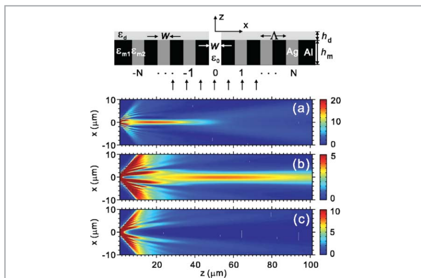
Fig. 59 Calculations of light transmission through a nano-hole surrounded by concentric rings of Al and Ag. For these calculations the incident wavelength is 539 nm, h_m = 360 nm and \Lambda = 380 nm. The thickness of the dielectric over the metal is h_d = 80 (a), 100 (b) and 120 (c) nm. (Reprinted with permission from ref. 170. Copyright 2006, American Institute of Physics.)
