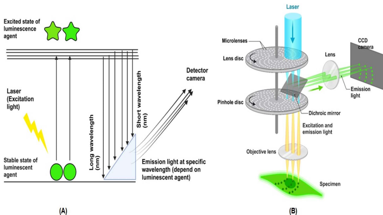
Fig. 1 Principal of FI using luminescence agent such as green fluorescence probe (GFP) and confocal microscopy. (A), a schematic of principles of FMI, (B), fluorescence confocal microscopy and various stages of FI and recording image from sample.
