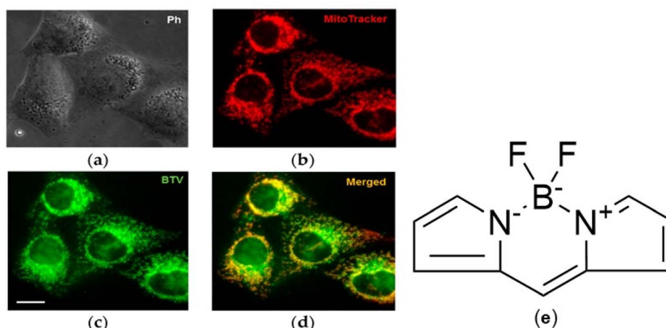
Fig. 2 Fluorescence microscopic images of BODIPY-based viscosity probe (BTV) in HeLa cells with stained with MitoTracker. DeepRed. Images were taken with a 40× objective. Scale bar represents 20 μm. (a) Phase contrast; (b) MitoTracker DeepRed; (c) BTV; (d) merged of MitoTracker DeepRed and BTV. Adapted from ref. 65 (under the terms of the Creative Commons CC BY 4.0 license) (e) chemical structure of BODIPY dye.
