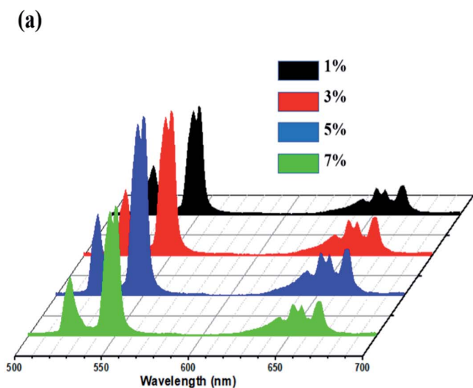
Fig. 5 (a) UC emission spectra of a series of \text{LiZnPO}_4:0.5\% \text{Ho}^{3+}/x\% \text{Yb}^{3+} phosphors with different \text{Yb}^{3+} concentrations ( x = 1, 3, 5 and 7 \text{ mol}\% ). (b) Energy level diagram illustrating thermally promoted ET from \text{Yb}^{3+} to \text{Er}^{3+} ions.
