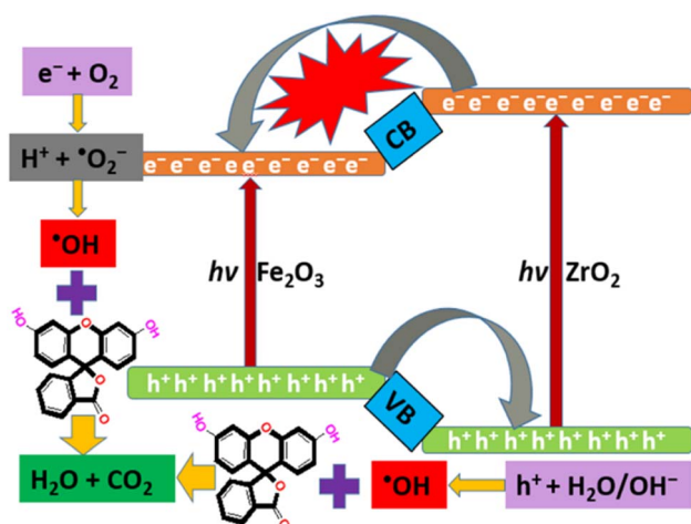
Fig. 10 Proposed photocatalytic mechanism showing the electron-hole generation and subsequent photocatalytic reactions.
