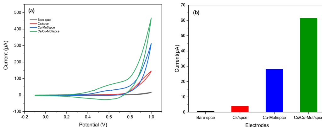
Fig. 6 (a) CVs of the bare SPCE, Cs/SPCE, Cu-MOF/SPCE and Cs/Cu-MOF/SPCE in 0.05 M KOH containing 200 \mu\text{M} glucose at scan rate 50 \text{ mV s}^{-1} . (b) Comparison of the current oxidation peak of glucose at different sensors.
