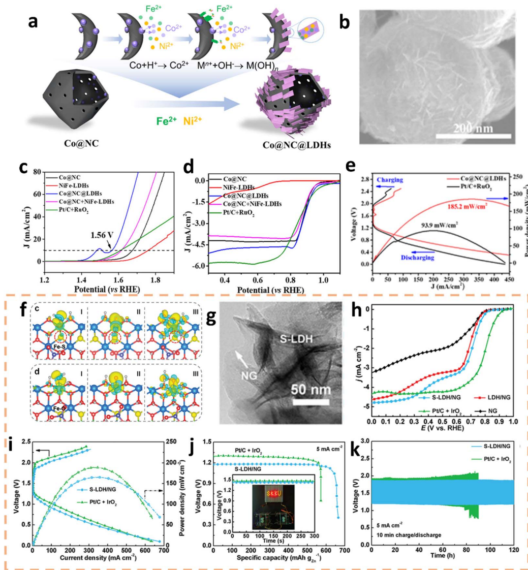
Fig. 13 (a) Schematic representation of the synthesis process for Co@NC@LDHs. (b) SEM images of Co@NC@LDHs. LSV curves for the OER (c) and ORR (d) of various catalysts including Co@NC, NiFe-LDHs, Co@NC@LDHs, Co@NC + NiFe-LDHs, and Pt/C + RuO 2 . (e) Polarization and power density profiles for ZABs equipped with Co@NC@LDHs and Pt/C + RuO 2 catalysts. Reproduced with permission from ref. 182 Copyright 2023 Wiley-VCH. (f) Charge density difference mappings for intermediate species at the zigzag edge of the Fe–S and Fe–O sites. (g) TEM image of S-LDH. (h) ORR polarization curves of S-LDH/NG and other samples. Comparison of S-LDH/NG and Pt/C + IrO 2 -based ZABs, showcasing charge/discharge polarization, power density (i), specific capacity (j), and cycling stability (k). Reproduced with permission from ref. 184 Copyright 2023, Wiley-VCH.
