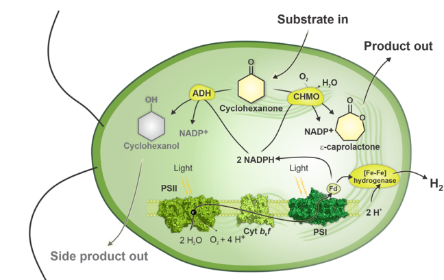
Fig. 1 Concept of the study. Engineered Chlamydomonas that expresses CHMO converts fed cyclohexanone to \epsilon -caprolactone by utilising photosynthetically produced O 2 and reductants. Innate alcohol dehydrogenases (ADHs) compete for the substrate, cyclohexanone, and convert it to cyclohexanol. Innate [Fe–Fe]-hydrogenases photoproduce H 2 under microoxic conditions utilising photosynthetically reduced ferredoxin (Fd).
