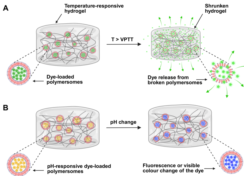
Fig. 1 Schematic illustrations of NIPAM-based hydrogels (HPCs) embedding dye-loaded polymerosomes (A) after heating above the VPTT of PNIPAM, and (B) upon pH change of the outer environment. Created in BioRender. Kraus, M. (2025) https://BioRender.com/u06z774 .
