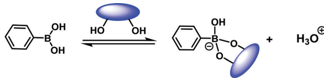
Scheme 5 The reversible interaction between boronic acid derivatives and diols-containing molecules.
