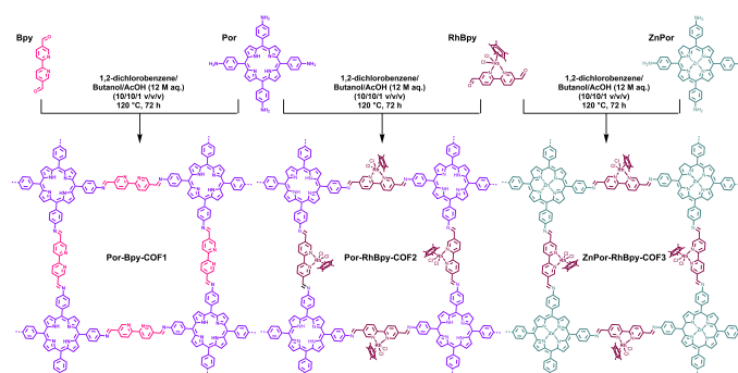
Scheme 1 Synthesis of Por-Bpy-COF1, Por-RhBpy-COF2, and ZnPor-RhBpy-COF3.
