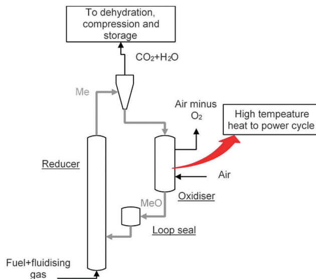
Fig. 12 Typical chemical looping combustion (CLC) process. The metal oxide oxygen carrier (MeO) is circulated between two fluidised reactors. In the reducer, the MeO gives up oxygen to the fuel to produce \text{CO}_2 and water. The reduced oxygen carrier (Me) is then carried over into a cyclone where the solid is separated from the gas phase and sent to an oxidiser where Me is regenerated, taking in oxygen from the air. The regenerated oxide MeO is then returned to the reducer for another cycle.
