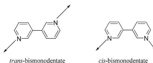
Scheme 2 cis - and trans -orientation of 3,3'-bipyridine as a bridging \mu -3,3'-bismonodentate ligand.
