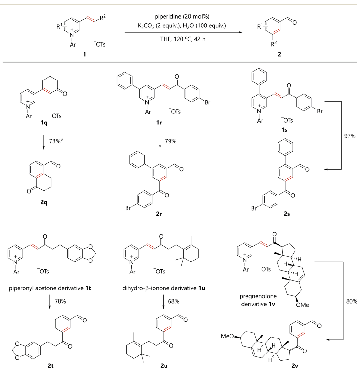
Scheme 2 Conversion of pyridiniums to various benzene derivatives using an amine catalyst. Pyridinium 1 (0.1 mmol), piperidine (0.02 mmol), K_2CO_3 (0.2 mmol), H_2O (10 mmol), and THF were stirred in a pressure tube under argon atmosphere. Ar = 2,4-dinitrophenyl. a The reaction was carried out at 40 °C for 16 hours.
