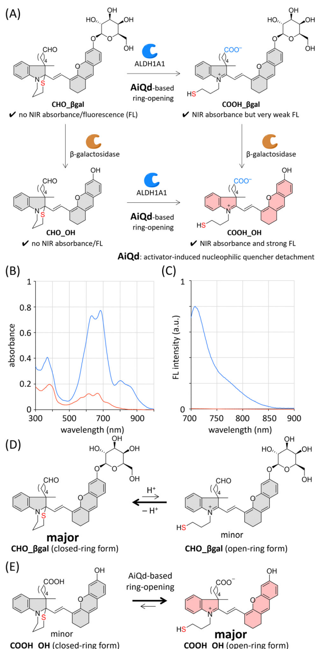
Fig. 2 (A) Dual-responsive AND-type fluorescent probe CHO_βgal . (B) Absorption and (C) fluorescence spectra of CHO_βgal (red) and COOH_OH (blue) in PBS (20 μM, pH 7.4, 1% DMSO). \lambda_{\text{ex}} = 680 nm. The equilibrium between open- and closed-ring forms of (D) CHO_βgal and (E) COOH_OH .
