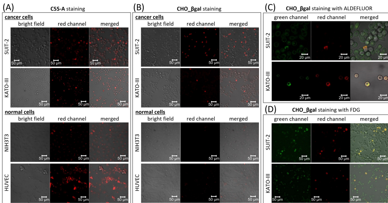
Fig. 4 Confocal laser scanning microscope images of SUIT-2, KATO-III, NIH3T3, and HUVEC cells stained with (A) CSS-A ( 1 \mu\text{M} ) or (B) CHO_βgal ( 20 \mu\text{M} ) without a washing step. Confocal laser scanning microscope images of SUIT-2 and KATO-III cells co-stained with CHO_βgal ( 20 \mu\text{M} ) with (C) ALDEFLUOR ( 1 \mu\text{M} ) or (D) FDG ( 20 \mu\text{M} ). Green channel: \lambda_{\text{ex}} = 488 \text{ nm} ( \lambda_{\text{det}} = 500\text{--}600 \text{ nm} ); red channel: \lambda_{\text{ex}} = 633 \text{ nm} ( \lambda_{\text{det}} = 647\text{--}759 \text{ nm} ).
