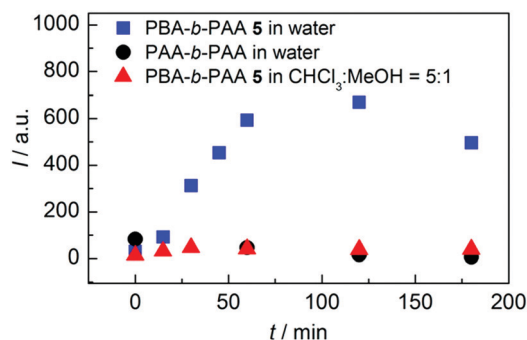
Fig. 26 Evolution of the emission intensity at \lambda_{em} = 420 nm as a function of sonication time of PBA- b -PAA dispersed in water (square) or in solution (triangle) and PAA- b -PAA in aqueous solution (circle). 58 Fig. 26 is reprinted with permission from ref. 58, Copyright 2016 American Chemical Society.
