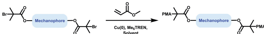
Fig. 16 General procedure for the preparation of mechanophore-linked PMA based on SET-LRP route using \alpha -bromo- \alpha -methylpropionylbifunctionalized mechanophore as an initiator.
