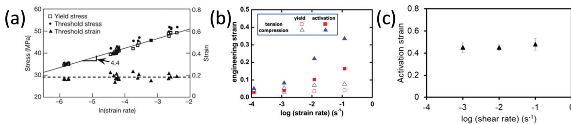
Fig. 31 Activation (strain or stress) threshold for SP-linked crosslinked PMMA as a function of strain rate: (a) Threshold (color) stress, yield stress and threshold strain as a function of strain rate reported by Davis et al. , 35 (b) Yield- and activation strain as a function of strain rate in tension test and compression test as described by Kim et al. , 176 (c) Activation strain as a function of shear rate, plotted using the values reported by Kingsbury et al. 177 (a) is reprinted with permission from ref. 35, Copyright 2009 Springer Nature. (b) is reprinted with permission from ref. 176, Copyright 2015 American Chemical Society. (c) is reprinted with permission from ref. 177, Published by The Royal Society of Chemistry ( https://creativecommons.org/licenses/by/3.0/ ).
