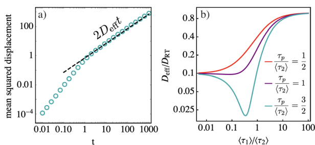
Fig. 2 (a) Mean squared displacement of an active run-and-tumble particle intermittently switching to a passive phase. Active durations are drawn from a gamma distribution (27) with shape index \gamma = 3 . The dashed line shows theoretical prediction based on the effective diffusion coefficient [i.e., eqn (24) with (28)], while circles show numerical simulation data. For simplicity, the passive phases have deterministic duration \langle \tau_2 \rangle = 1/2 . Remaining parameters used are v = 1 , D = 1 , \tau_p = 0.5 . (b) Effective diffusivity rescaled with D_{\text{RT}} \equiv v^2 \tau_p as a function of the ratio of active durations to passive durations, again for the case when active durations are drawn from a gamma distribution (27) with shape index \gamma = 3 . In this case, we have set D/D_{\text{RT}} = 0.1 , so that passive phases are slow compared to the active motion.
