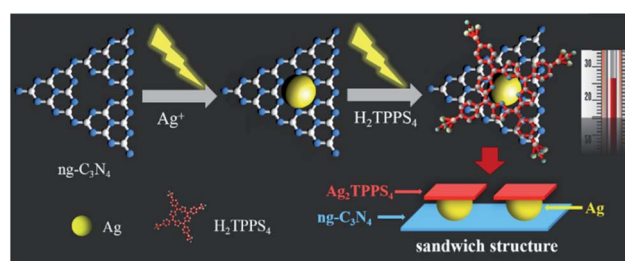
Scheme 1 The photocatalytic synthesis processes of Ag 2 NPs/ng-C 3 N 4 and Ag 2 TPPS 4 /AgNPs/ng-C 3 N 4 .
