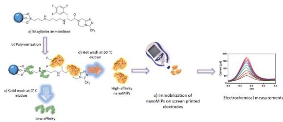
Scheme 1 Preparation and elution of high affinity sitagliptin nanoMIPs (a) to (d) and (e) their use in the fabrication of sitagliptin sensors.
