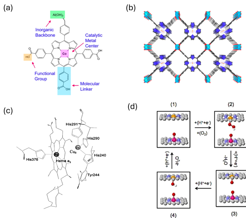
Fig. 5 (a) and (b) Coordination entity for constructing Al 2 (OH) 2 TCPP-Co MOF. Adapted from ref. 55 with permission. (c) Cytochrome- C oxidase enzyme. Adapted from ref. 58 with permission. (d) Illustration of the bio-mimic prototype catalyst capable of circumventing the scaling relations.
