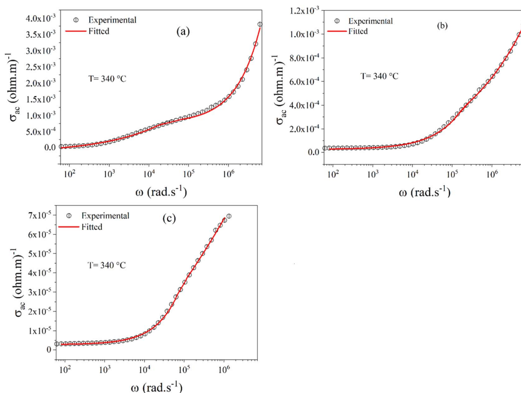
Fig. 11 AC conductivity versus frequency at T = 340\text{ }^\circ\text{C} for: (a) BZT, (b) BSmZT (c) BLaZT.
