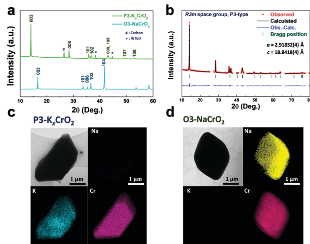
Fig. 2 (a) Comparison of the XRD patterns for the P3-K x CrO 2 electrode and O3-NaCrO 2 powder. (b) Profile-matched XRD patterns of P3-K x CrO 2 using Rietveld refinement ( R_p = ~1.65%, R_i = ~1.28%, R_f = ~2.07%, and \chi^2 = ~7.43%). TEM images and the corresponding EDX mapping of (c) P3-K x CrO 2 and (d) O3-NaCrO 2 .
