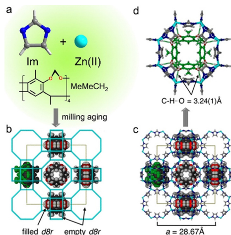
Fig. 11 The mechanochemical synthesis and structural features of \text{MeMeCH}_2@rho\text{-Zn}_{16}(\text{Im})_{32} . (a) Imidazole, zinc salt, and \text{MeMeCH}_2 as precursors of materials. (b) Wireframe and (c) ball-and-stick representation of the \rho\text{-ZnIm}_2 framework, occupied by \text{MeMeCH}_2 . (d) Top view of the \text{MeMeCH}_2@d8r motif. Adapted from ref. 64 with permission of the American Chemical Society, Copyright 2018.
