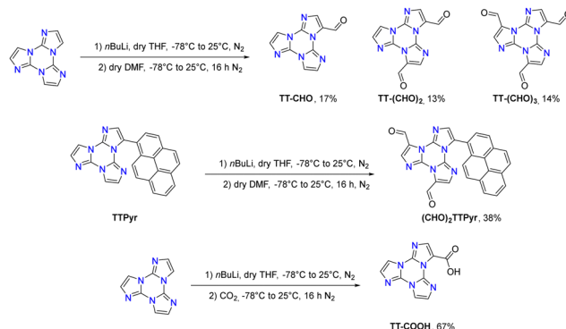
Scheme 8 Synthesis of TT derivatives by formylation.
