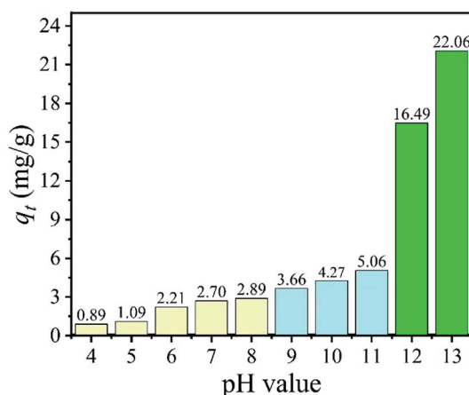
Fig. 8 The effect of pH value on Li^+ adsorption ( C_0 : 24 mM LiCl, adsorbent: 0.1 g, volume: 50 mL, T : 25 ^{\circ}C ).
