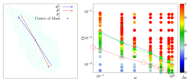
Fig. 11 (left) A typical cluster is shown. The eigen direction \bar{\theta}^{\text{ei}} (blue arrow) corresponding to the largest eigenvalue of the gyration tensor and the velocity direction \bar{\theta}^v (red arrow) of the cluster are depicted. (right) The \alpha – \kappa phase diagram in the low density \rho = 0.01 , with the \cos \Delta_\theta color coded also shown.
