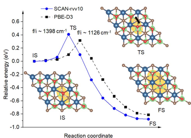
Fig. 8 The energy paths, calculated with SCAN-rvv10, with a reference via PBE-D3, are shown for the dissociation of H 2 O initiated at O v sites. It also includes the geometries of adsorption/initial state (IS), transition state (TS), and final state (FS). The orange background highlights the active region of H 2 O on the surface for a top view. The imaginary frequencies denoted as "f/i" are provided for transition states. The black arrow indicates the vibrational direction of the dissociated hydrogen atom at the TS.
